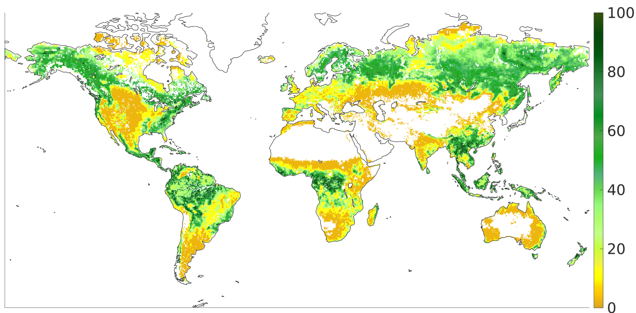
Figure 10. Spatial bias ( \text{Mg ha}^{-1} ) related to the logistic fit between the AGB values from CCI 2018 and the SMOS L-VOD.
