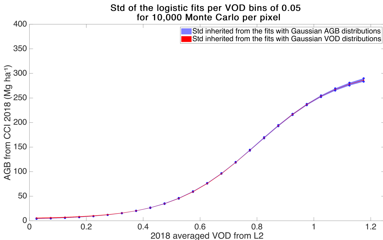
Figure 11. Standard deviation ( \text{Mg ha}^{-1} ) of the 10,000 Monte-Carlo draws for a Gaussian AGB distribution per pixel (blue) and a Gaussian L-VOD distribution per pixel (red).
