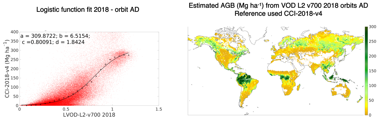
Figure 5. The left panel shows the parameter values and the mean logistic fit between the CCI 2018 AGB map version 4 and the VOD from SMOS L2 products filtered and averaged over 2018. The right panel is the estimated AGB in \text{Mg ha}^{-1} by applying the logistic function with the estimated a , b , c and d parameters to the 2018 averaged VOD
