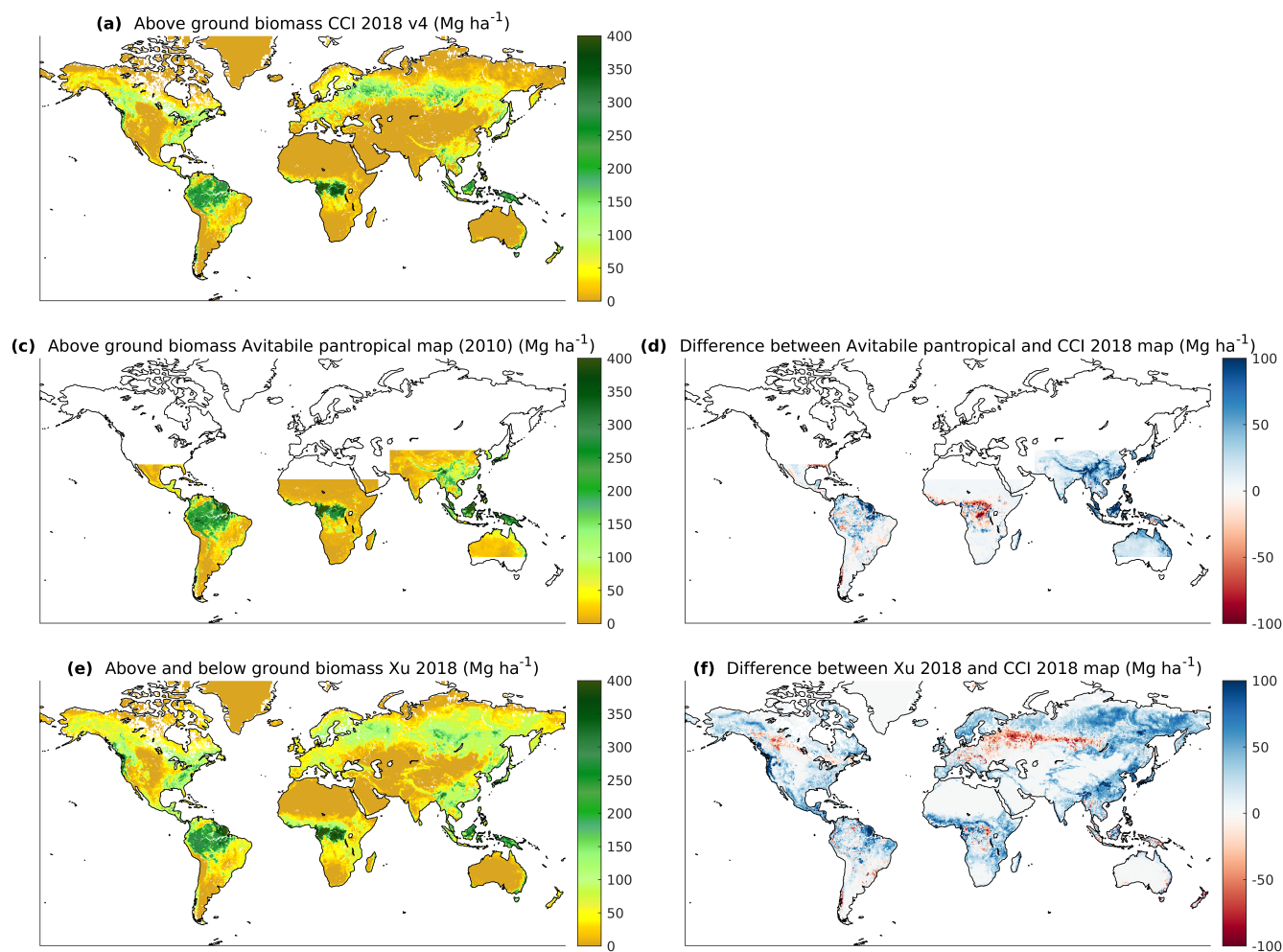
Figure 2. Reference maps used in this study and the spatial differences between them. (a) Above ground biomass from Santoro and Cartus (2023), (c) Above ground biomass from Avitabile et al. (2016), (d) Above ground biomass difference between Avitabile et al. (2016) minus Santoro and Cartus (2023), (e) Above and below ground biomass (BGB) in 2018 from Xu et al. (2021a), (f) Biomass difference between Xu et al. (2021a) minus Santoro and Cartus (2023). All units are in Mg ha -1 and all maps are resampled to the EASE 2 grid at 25 km
