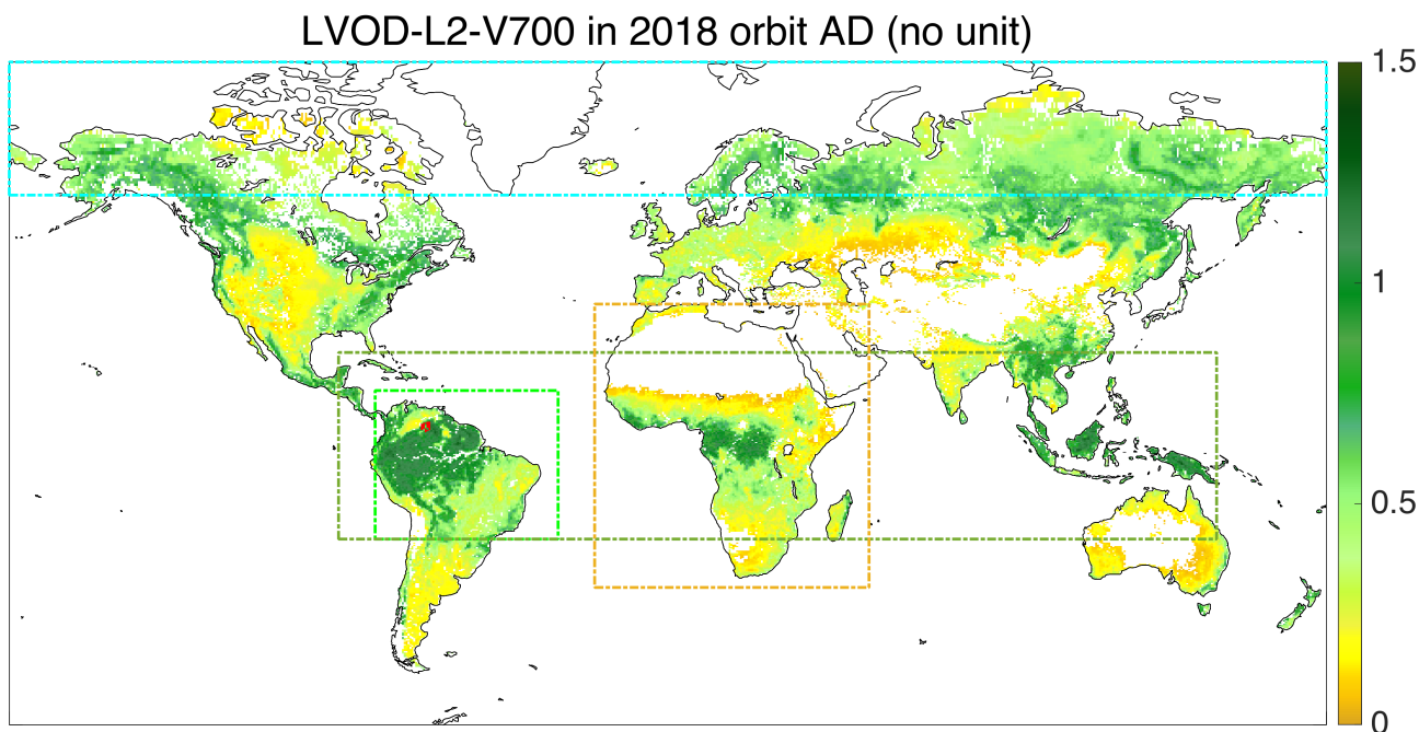
Figure 1. L-VOD from SMOS L2 v700 products averaged over 2018. Ascending and descending orbits are mixed. Values where RFI contamination is higher than 20 % or where the Chi2\_P is lower than 5 % are filtered out. Pixels with an AGB reference value equals to 0 are also filtered out and outliers are discarded. The colored rectangles show the extent of the different regions considered in the study
