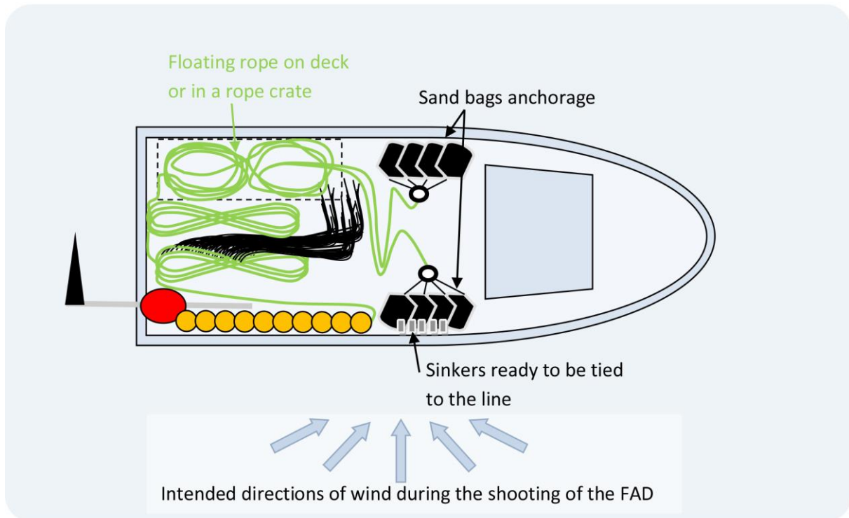
Figure 25: Correct layout on the deck of a 9 m (30 ft.) fishing boat for deployment on starboard side.
