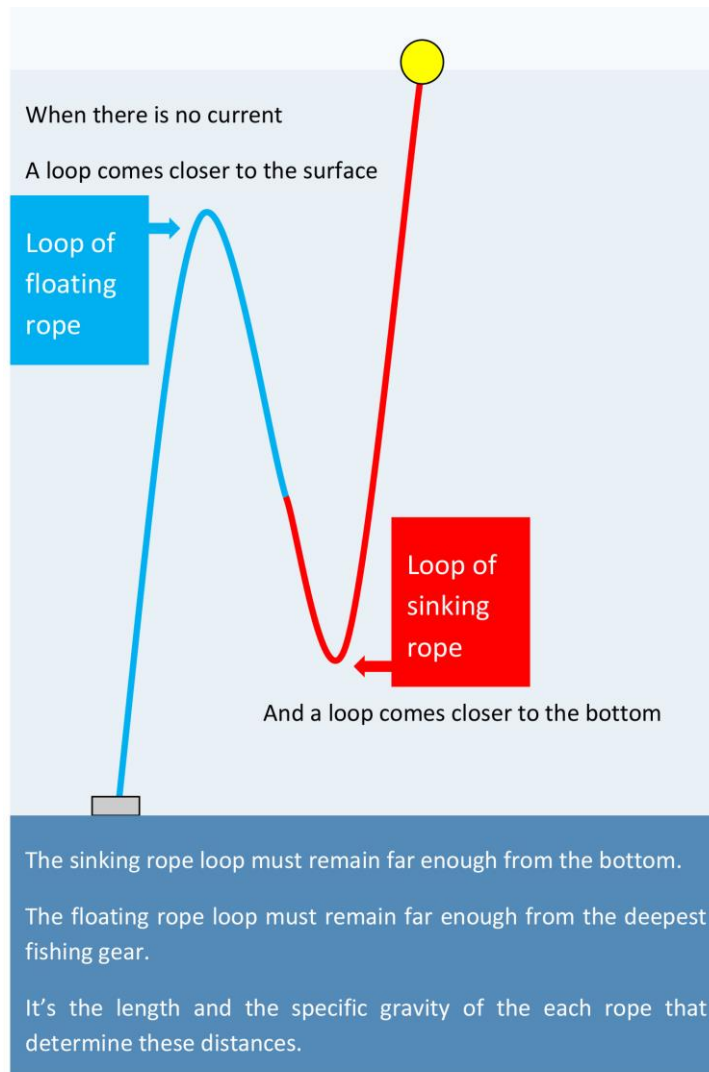
Figure 9: When there is no current, the two loops of the catenary curve.
