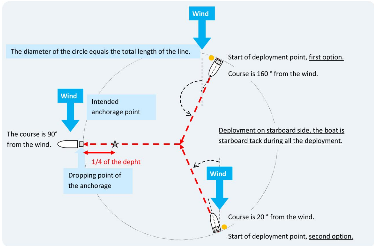
Figure 28: Courses during the deployment. Start points and dropping points when there is no current.
