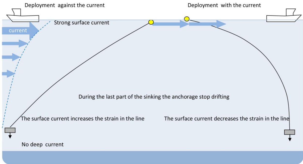
Figure 26: Avoid deploying straight against the current.
