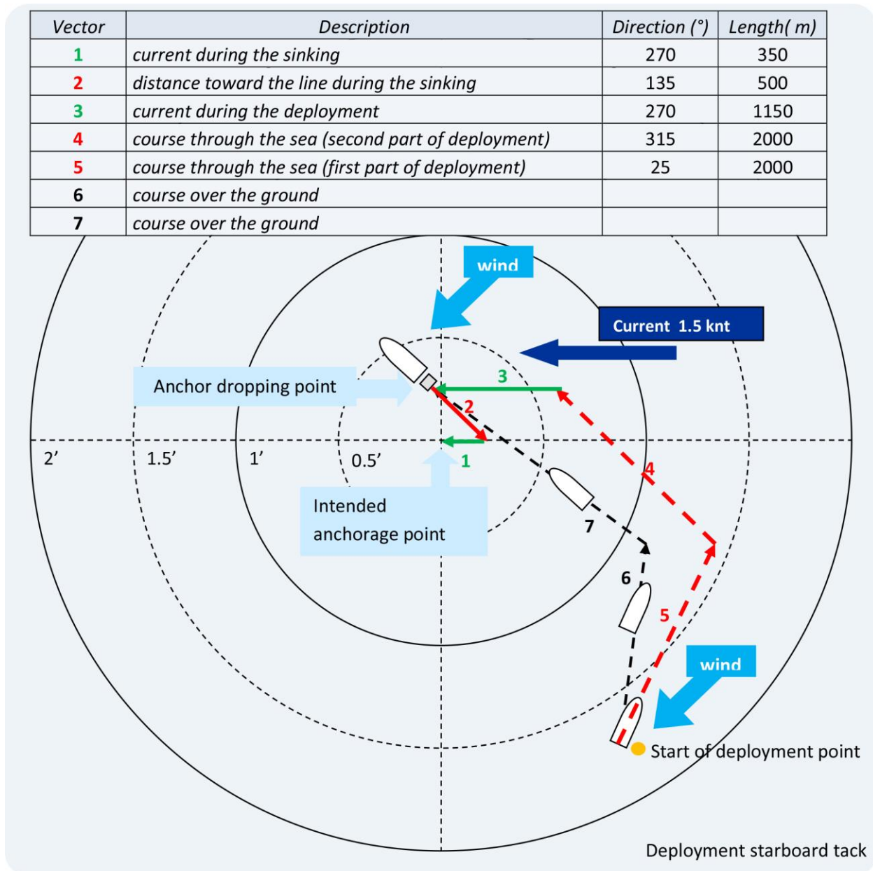
Figure 29: Courses during the deployment. Example with a NE wind and a W current (1.5knt).
