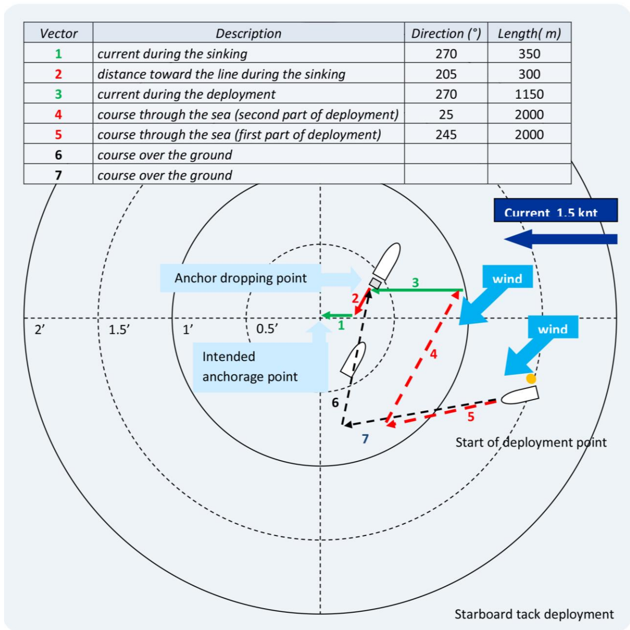
Figure 30: Courses during the deployment. 2 nd Example with a NE wind and a W current (1.5knt).
