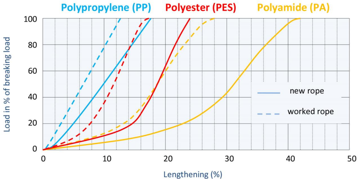
Figure 15: The lengthening of ropes.
