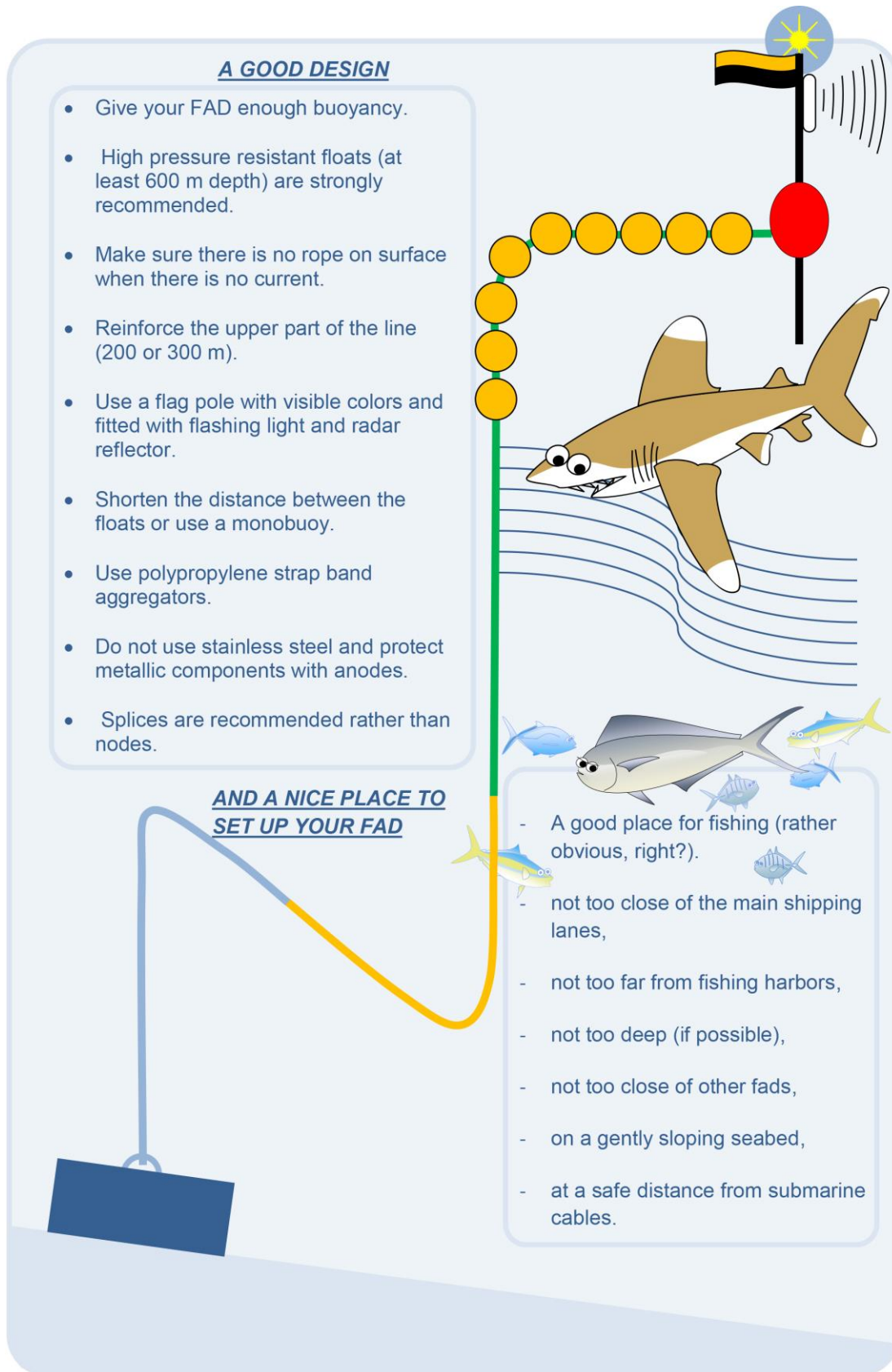
Figure 5: A Good FAD Design.
