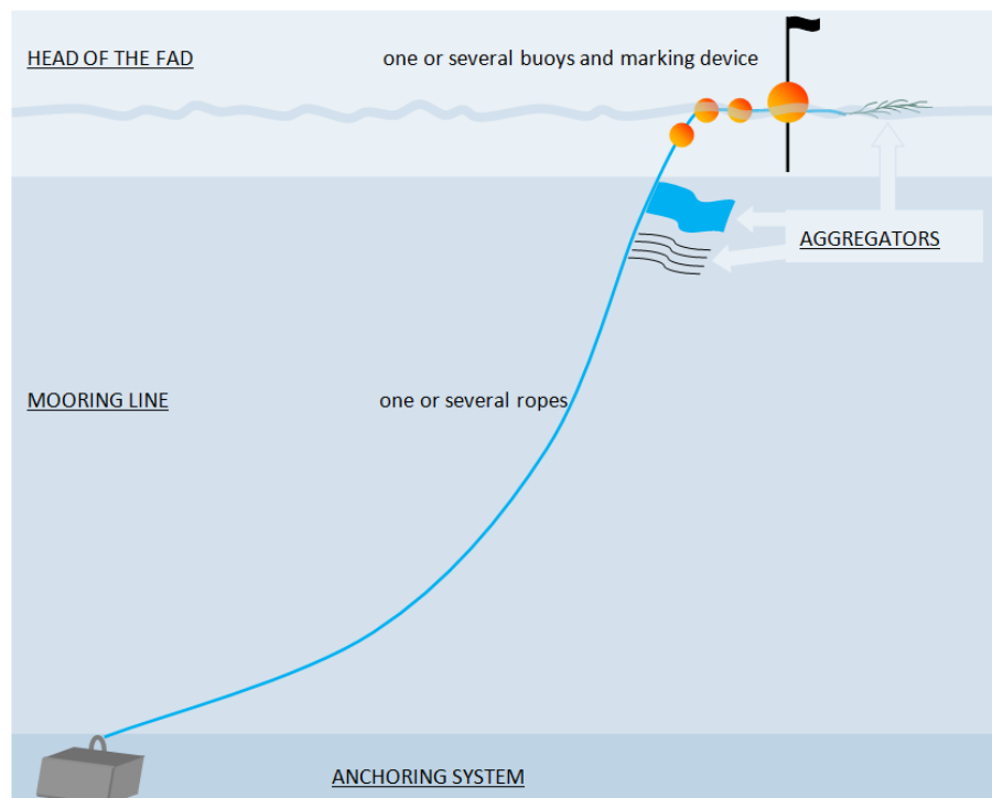
Figure 1: Diagram of a FAD.
