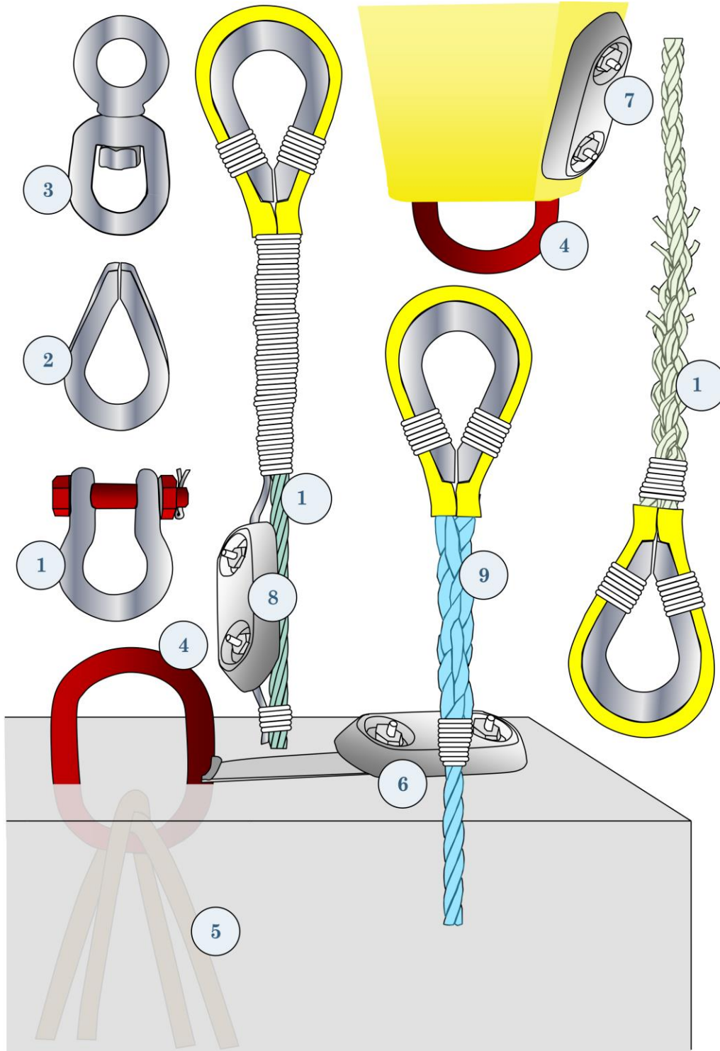
Figure 18: Metal components of a FAD.
