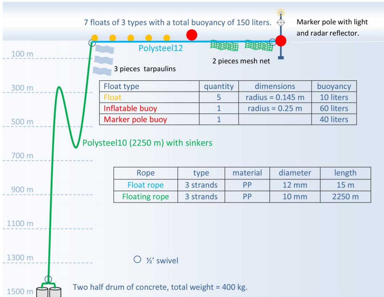
Figure 23: CARIFICO Project FAD.
