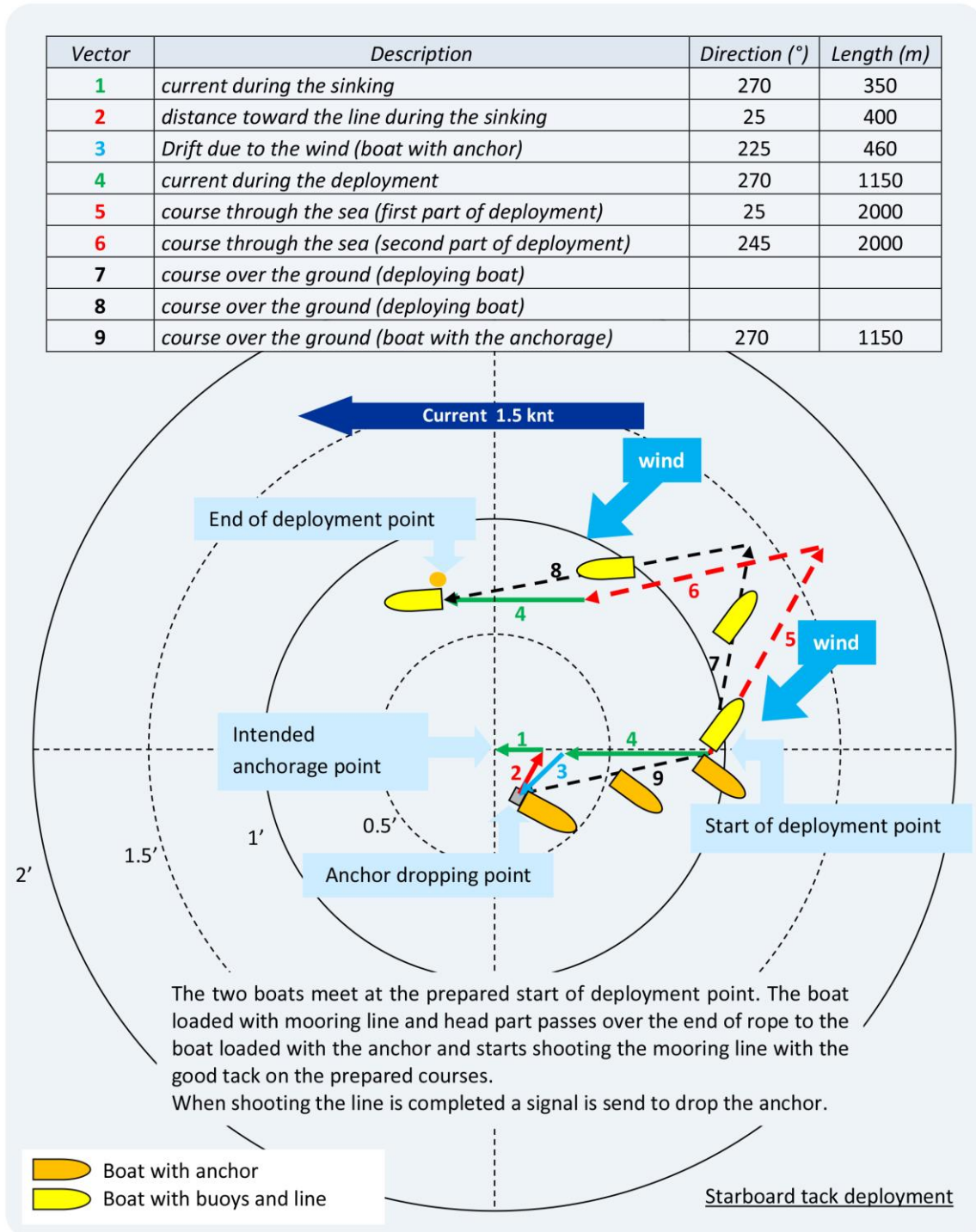
Figure 31: Dual boat deployment. Example with a NE wind and a W current (1.5knt).
