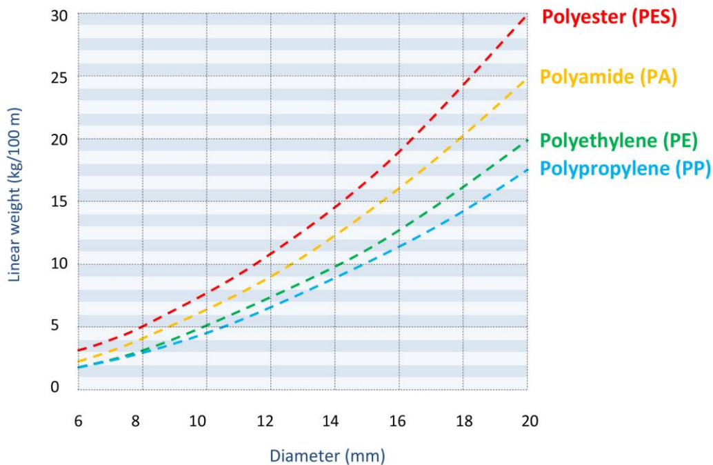
Figure 11: The linear weight of a rope.
