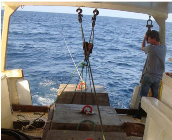
Photo 19: Large stern door in the transom, the concrete blocks are loaded directly on the deck.
