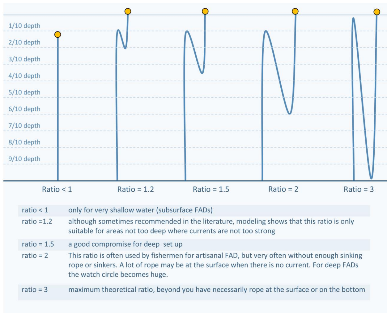
Figure 14: The length to depth ratio.
