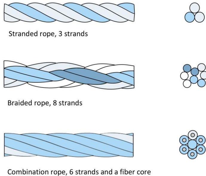
Figure 10: Types of ropes used in FAD mooring lines.
