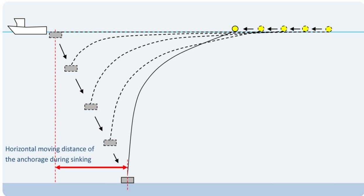
Figure 27: In a straight deployment the anchorage moves towards the buoy during the sinking.
