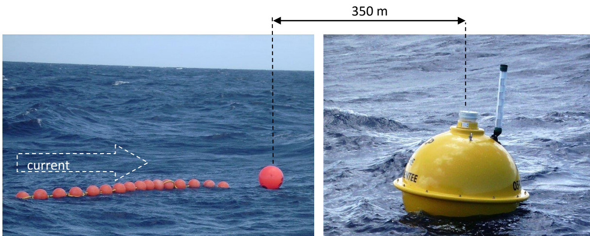
Photo 16: First head of a Two-Headed FAD.
