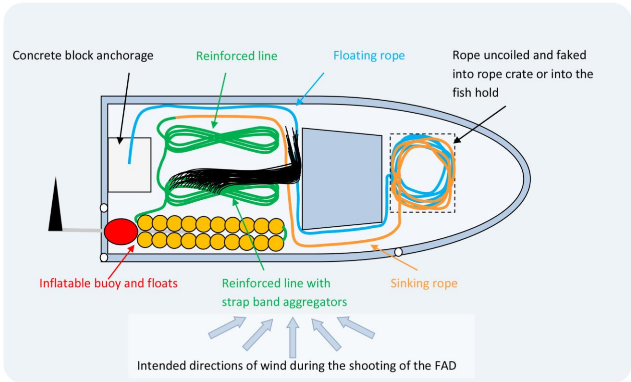
Figure 24: Correct layout on the deck of an 11 m (36 ft.) fishing boat for deployment on starboard side.
