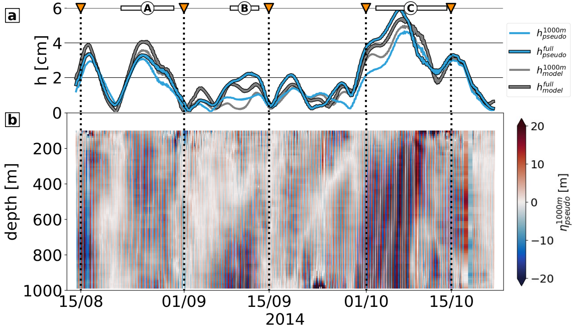
Figure 11. (a) Semidiurnal amplitude for the pseudo glider steric height h_{pseudo}^{1000m} (blue), the full-depth pseudo glider steric height h_{pseudo}^{full} (blue with black outlines), and the full-model steric height h_{model}^{1000m} for the upper 1000 m (gray) and h_{model}^{full} for the full-depth range (gray with black outlines). Here, we use a two-mode approximation to calculate h_{pseudo}^{full} . (b) Pseudo glider vertical displacements \eta_{pseudo}^{1000m} which are ultimately used to compute h_{pseudo}^{1000m} and h_{pseudo}^{full} .
