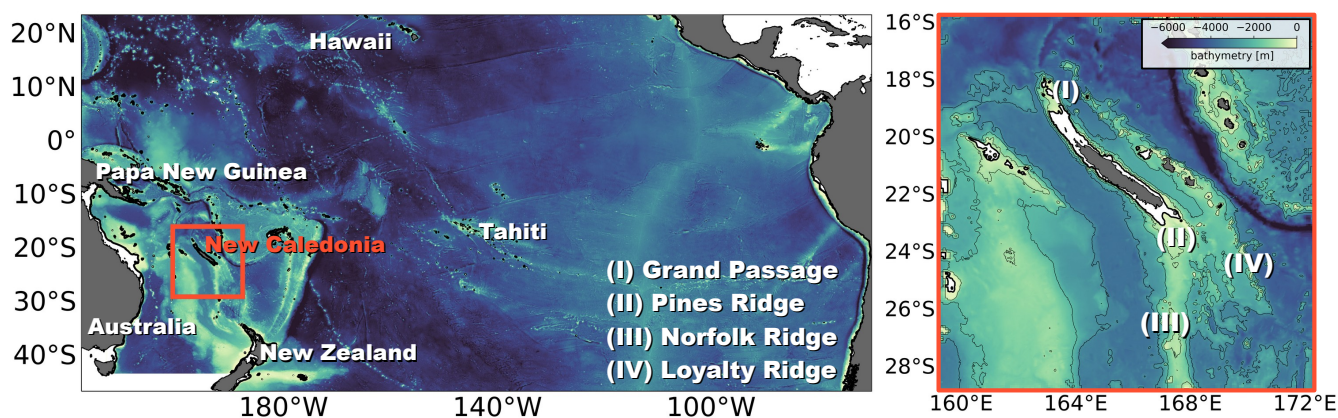
Figure 1. New Caledonia is located in the southwestern tropical Pacific, an area of complex bathymetry with continental shelves, shelf breaks, large- and small-scale ridges, and seamounts. It is subject to strong internal tide generation associated with the major bathymetric features, i.e. (I) Grand Passage, (II) Pines Ridge, (III) Norfolk Ridge, and (IV) Loyalty Ridge.
