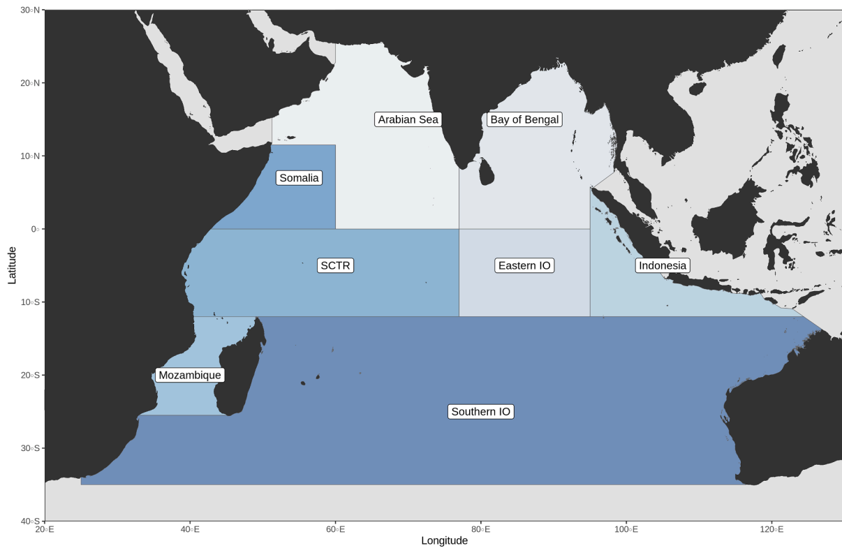
Fig. 1. Map of the different areas considered in the study. IO: Indian Ocean. SCTR: Seychelles-Chagos Thermocline Ridge.
