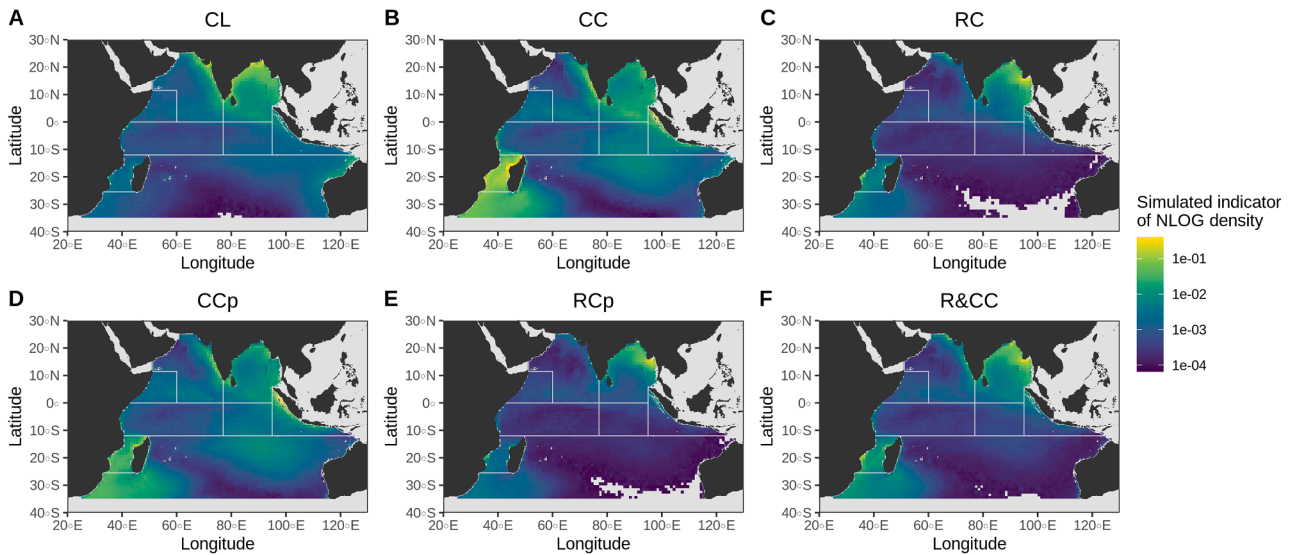
Fig. 4. Simulated density of NLOGs averaged over 2000–2019 for the different weighting scenarios. Maximum value was set to 1 and values below 10^{-4} were discarded. CL: Coastline Length; CC: Coastal forest Cover; RC: River forest Cover multiplied by river discharge; CCp: Coastal forest Cover multiplied by precipitations; RCp: River forest Cover multiplied by river discharge and by precipitations; R&CC: River plus Coastal forest Cover.
