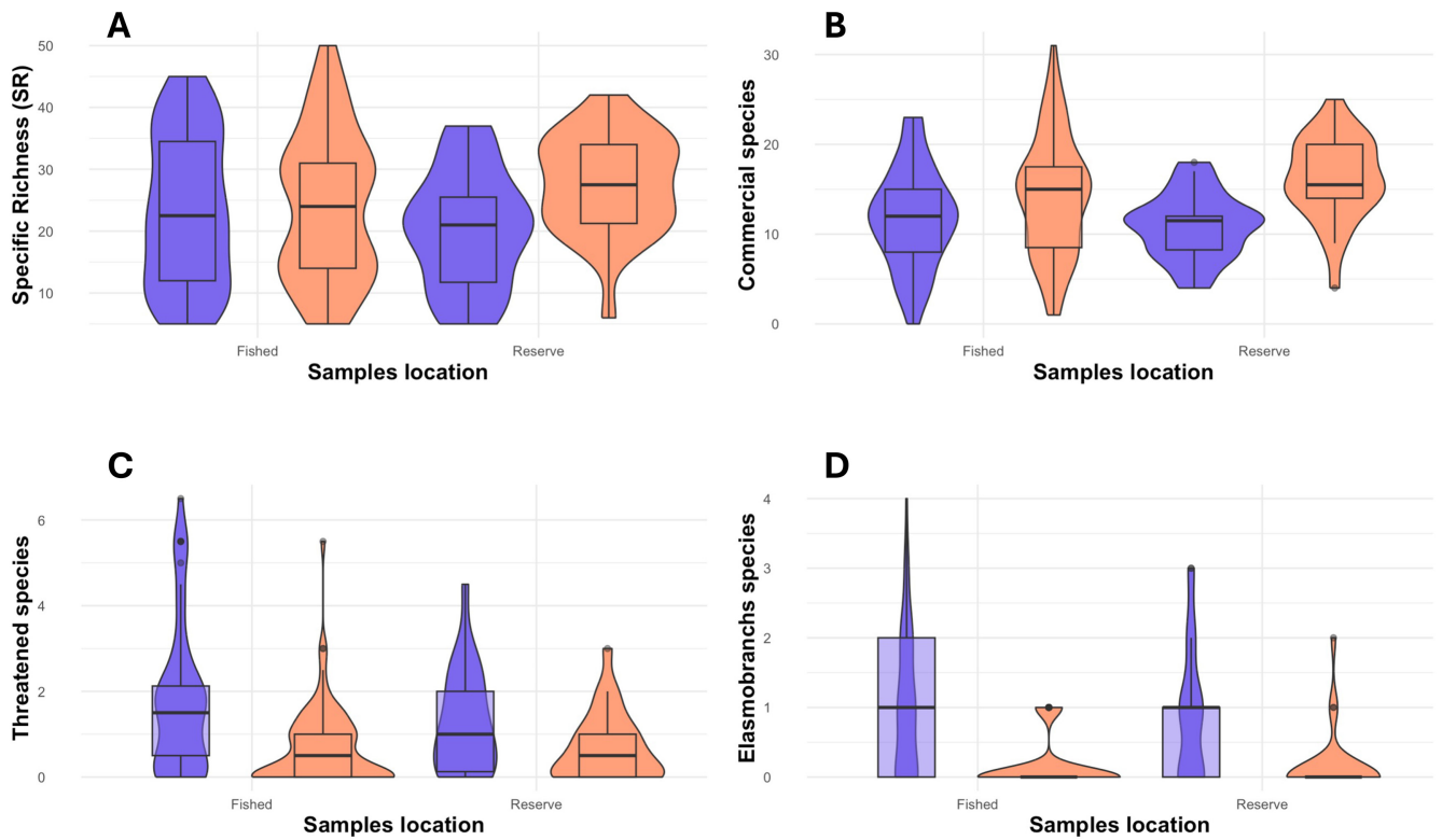
FIGURE 4 | Plots from the ANOVA with permutation using the avp function (package “lmPerm”) showing the distribution of the four biodiversity indices for continental and island eDNA samples from inside or outside marine reserves (Table 2). Shaded area represents the 95% confidence interval.
