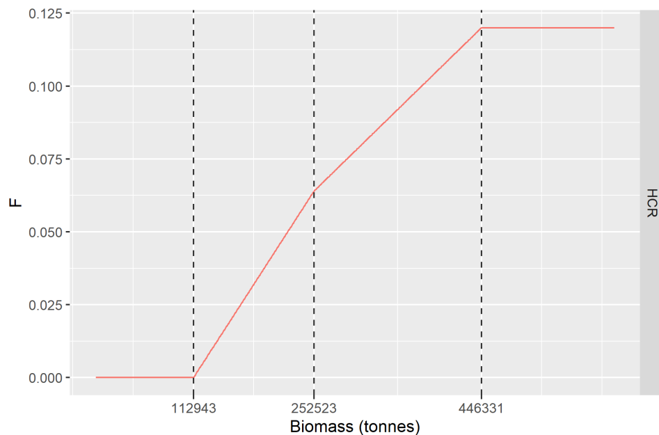
Figure 8.8.1. Proposed HCR. The biomass reference levels of biomass ( B_{1+} ) reported correspond to B_{loss(2018)} = 112\,943 t, MSY\ B_{trigger\_low} = B_{pa\_low} = 252\,523 t and MSY\ B_{trigger\_medium} = B_{pa\_medium} = 446\,331 t.
