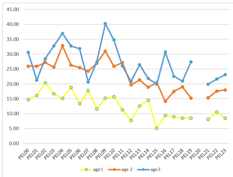
Figure 3.3.2.4: Bay of Biscay anchovy: evolution of mean weight at age (g) of anchovy along PELGAS series.
