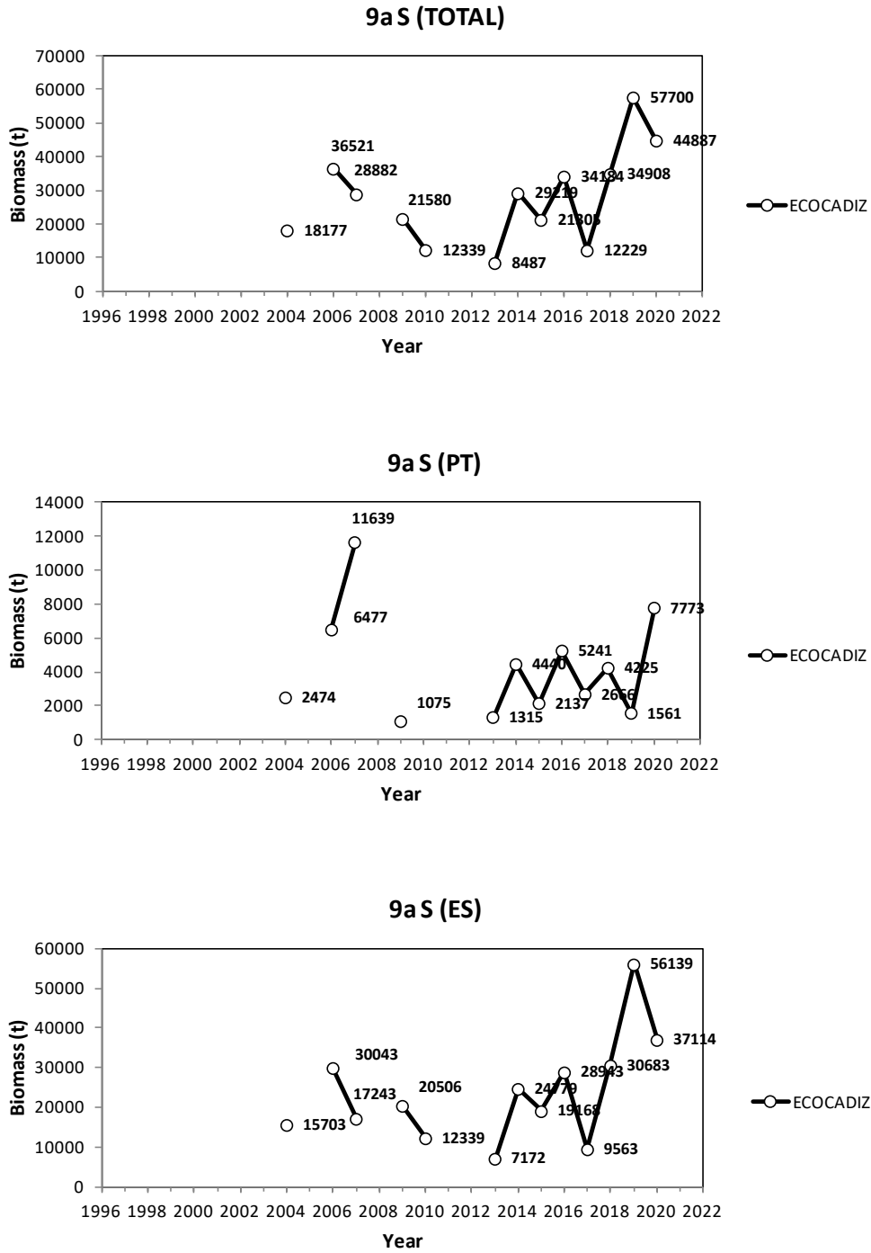
Figure 4.4.2.8. Anchovy in Division 9.a. Southern component. Subdivision 9.a South. ECOCADIZ survey series (summer Spanish acoustic survey in Subdivision 9.a South). Historical series of overall and regional (Portuguese, PT, and Spanish waters of the Gulf of Cadiz, ES) acoustic estimates of anchovy biomass (t). Note the different scale of the y-axis. ECOCADIZ 2021 and 2022 were not finally conducted.
