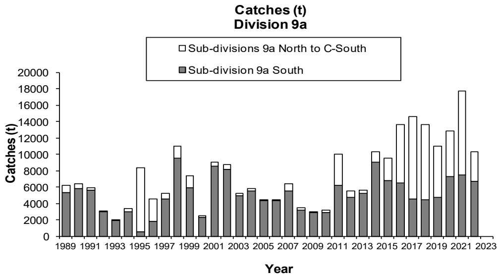
Figure 4.3.2.1.1. Anchovy in Division 9.a. Recent series of anchovy catches in Division 9.a (ICES estimates for 1989–2022, the period with data for all the subdivisions, all metiers are considered). Subdivisions are pooled in order to differentiate the anchovy fishery harvested throughout the Atlantic façade of the Iberian Peninsula (Western component: ICES subdivisions 9.a North, Central-North and Central-South) from the fishery in the Gulf of Cadiz (Southern component: Sub-division 9.a South), where both the stock and the fishery were mainly located during a great part of the time-series. Discards are considered as negligible all over the division, but since 2014 on estimates include the available discarded catches (see Section 4.3.3).
