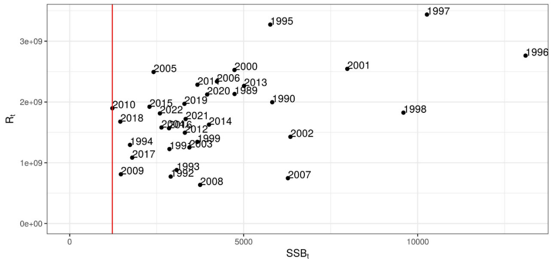
Figure 4.7.2.1. Anchovy in Division 9.a. Southern component. Estimated Stock Spawning biomass vs. Recruitment plot. Red line indicates the B_{lim} value ( B_{lim}=B_{loss}=SSB_{2010}= 1226.13 t).
