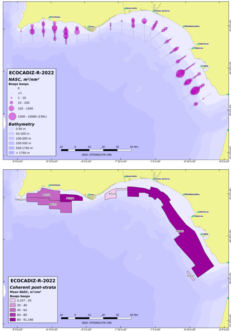
Figure 32. ECOCADIZ-RECLUTAS 2022-10 survey. Bogue ( Boops boops ). Top: distribution of the total backscattering energy (Nautical area scattering coefficient, NASC, in m 2 nm -2 ) attributed to the species. Bottom: distribution of homogeneous size-based post-strata used in the biomass/abundance estimates. Colour scale according to the mean value of the backscattering energy attributed to the species in each stratum.
