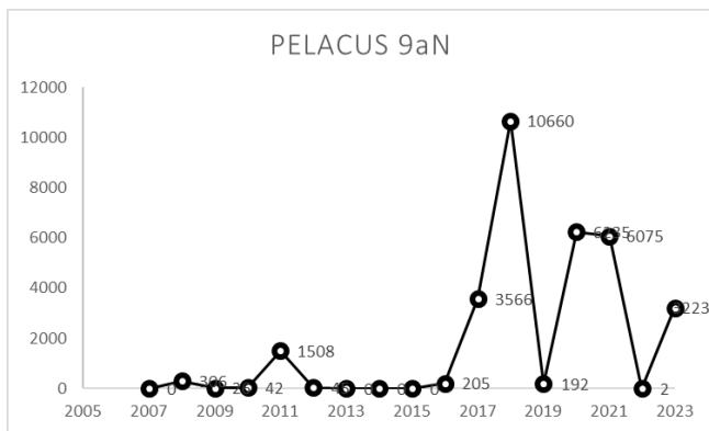
Figure 4.4.2.2. Anchovy in Division 9.a. Western component. Subdivision 9.a North. PELACUS survey series (spring Spanish acoustic survey in Subdivision 9.a North and Subarea 8c). Historical series of acoustic estimates of anchovy biomass (t) for the Subdivision 9.a North.
