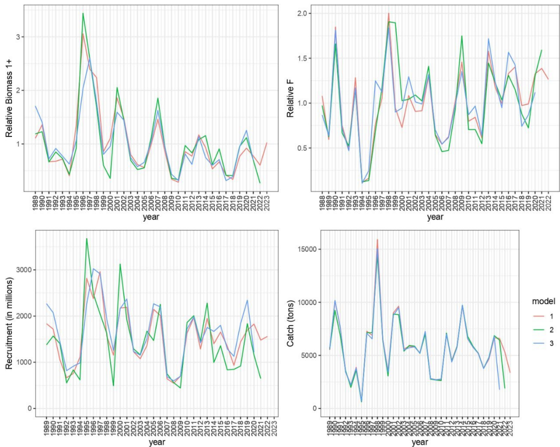
Figure 4.11.2.1: Anchovy in Division 9.a. Southern component. Comparison of estimates from different model implementations. 1: model used this year (pink); 2: model used last year (green); 3: model used in 2021 (blue). Annual model estimates for: relative abundance of individuals with more than one year of age (upper left), relative fishing mortality (upper right), recruitment (in million fish, bottom left) and catches (in numbers). Measures were summarized at the end of June each year, assuming that a year starts in July and ends in June of the next year.
