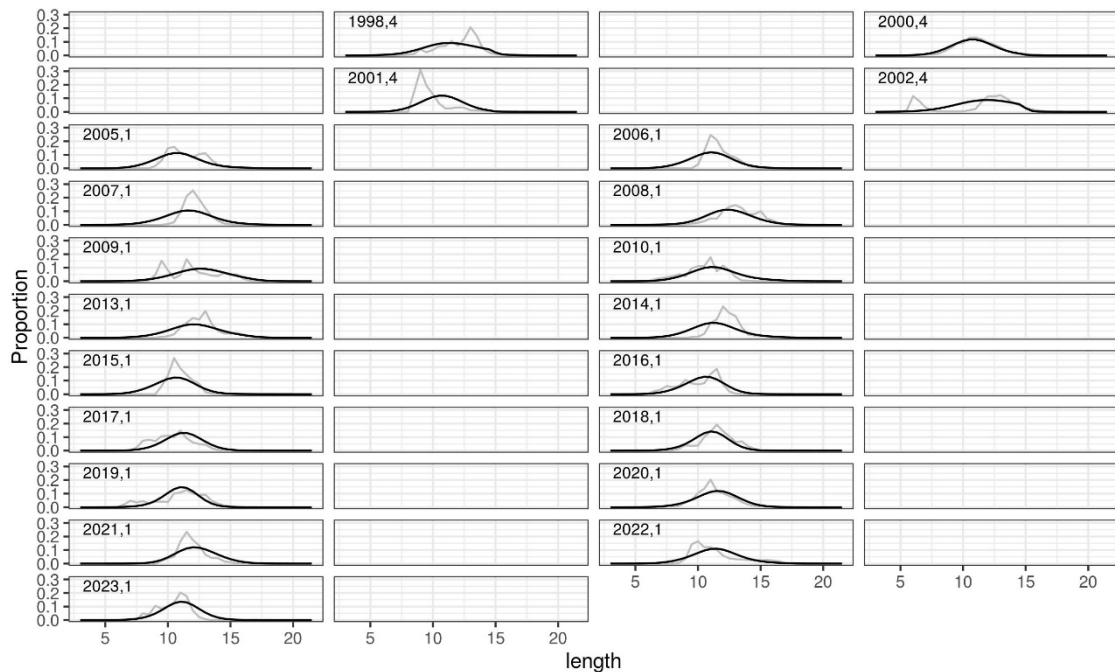
Figure 4.6.2.1.2.3. Anchovy in Division 9.a. Southern component. Comparison between observed and estimated catches length distribution for PELAGO survey from 1998 to 2023. Black lines represent estimated data while gray lines represent observed data. The number next to the year indicates the quarter. Note that the time of the survey in the model is assumed to be one quarter before it really happens; this assumption follows from the order of calculations in the model.
