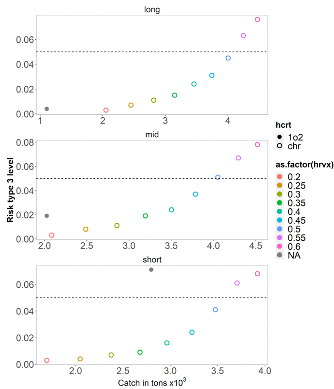
Figure 4.6.1.- Biological risk as Risk4.2.B lim : (maximum probability of falling below B_{lim} , y-axis) versus yield (catches in tonnes, x-axis) for the 1over2 advice rule (full circle) and the constant harvest rate rule (open circle) with different harvest rates (colours). The rows correspond to the temporal scales: the short-term (first 5 projection years), medium-term (next 5 projection years) and the long-term (last 10 years of the projection years). Black dashed line corresponds to the 0.05 risk.
