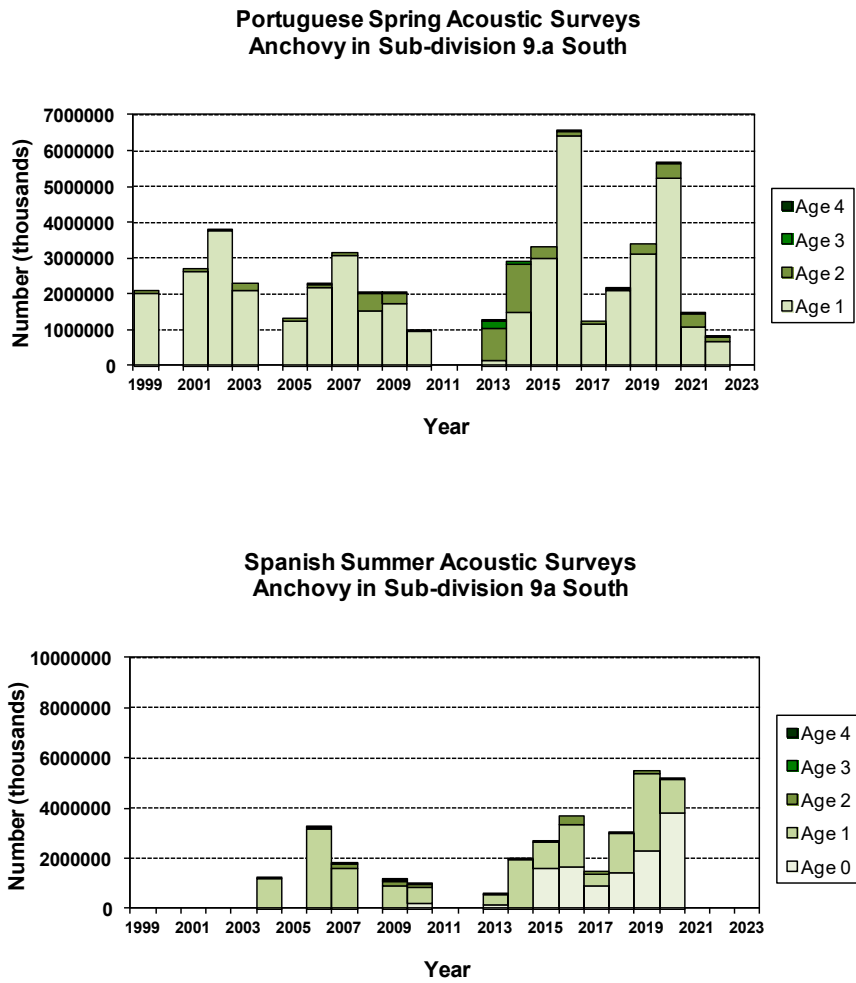
Figure 4.4.2.7. Anchovy in Division 9.a. Southern component. Subdivision 9.a South. Annual trends of the estimated population by age class from the Algarve + Gulf of Cadiz areas by the PELAGO Portuguese Spring (upper plot) and ECOCADIZ Spanish summer (lower plot) acoustic surveys ( ECOCADIZ 2021-07 was not finally conducted). Portuguese estimates until 2012 have been age-structured using Spanish ALKs from the commercial fishery in the second quarter in the year. The age structure estimated for the PELAGO 23 survey has not been included in the figure because some inconsistencies were found in the age readings.
