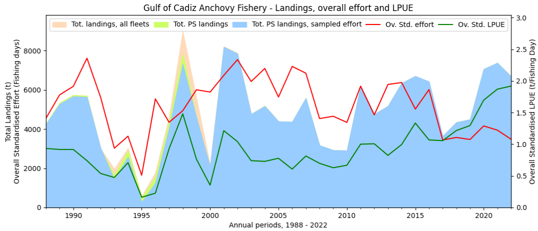
Figure 4.3.4.1. Anchovy in Division 9.a. Southern component. Subdivision 9.a South. Spanish purse-seine fishery (métier PS_SPF_0_0_0). Trends in Gulf of Cadiz anchovy annual landings, and purse-seine fleets’ standardised overall effort and lpue (1988–2022).
