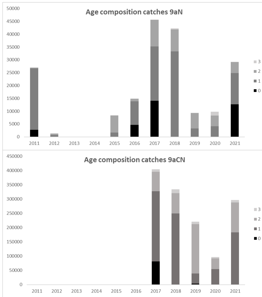
Figure 3-3 - Age composition of catches for the 9aN (upper panel) and 9aCN (lower panel) areas. No information available for the 9aCS sub-division.
