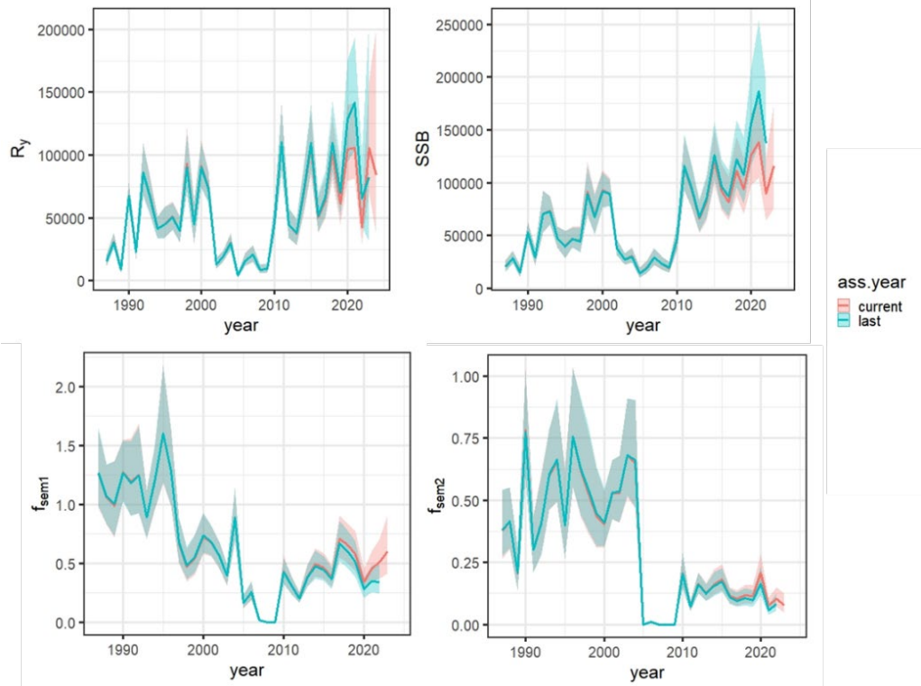
3.6.1.1: Bay of Biscay anchovy: Recruitment, SSB and fishing mortalities for first and second semester estimated in previous (last) and current assessments.
