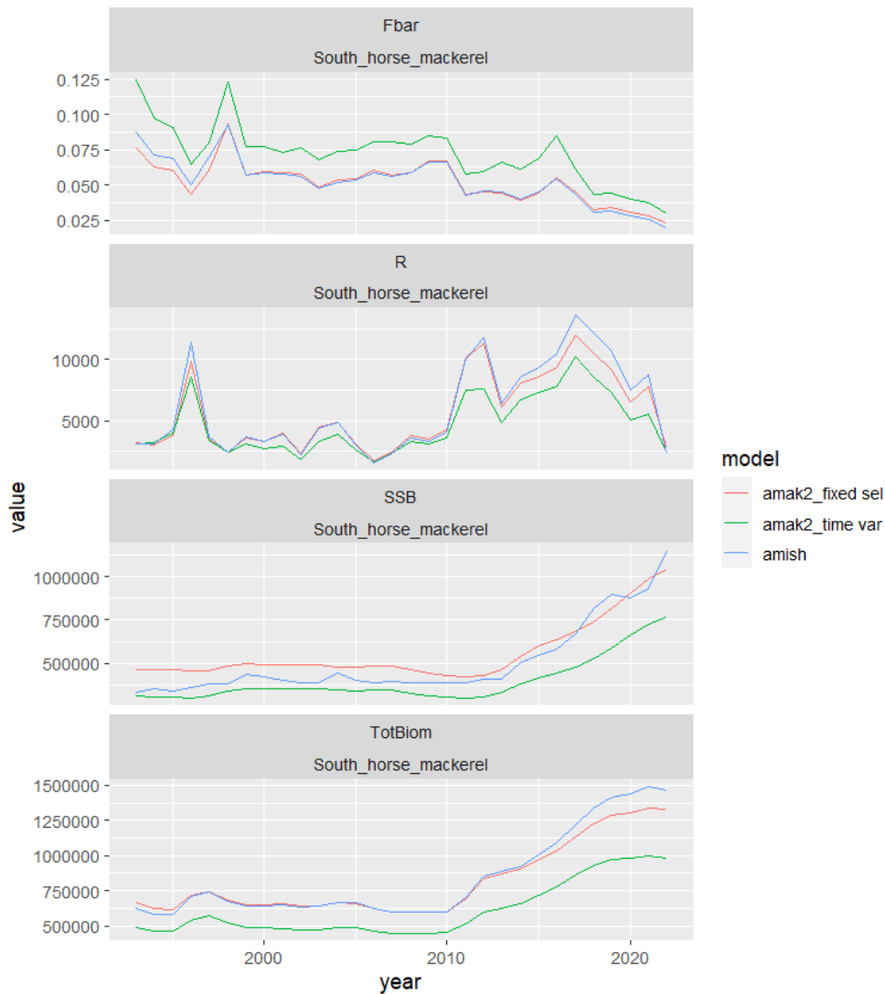
Figure 9.8.1.2. Horse mackerel in Division 9.a. Trajectories of F_{\text{bar}} , Recruitment, SSB and total biomass for the current assessment ( amish , blue line), time varying ( amak2_time var , green line) and fixed selectivity ( amak2_fixed sel , red line) exploratory assessment runs.
