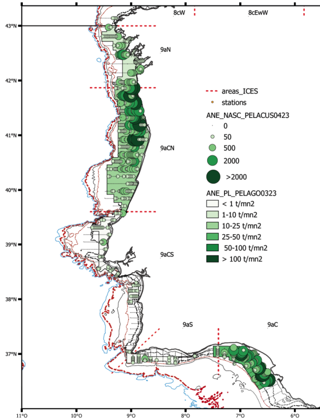
Figure 4.4.2.1. Anchovy in Division 9.a. Western component. Subdivision 9.a North. PELACUS 0423 survey (spring Spanish acoustic survey in Sub-division 9.a North and Sub-area 8c in 2023) and PELAGO 23 survey (spring Portuguese acoustic survey in Sub-divisions 9.a Central-North to 9.a South). Spatial distribution of energy allocated to anchovy (NASC coefficients in m^2/mn^2 ) in Division 9.a.
