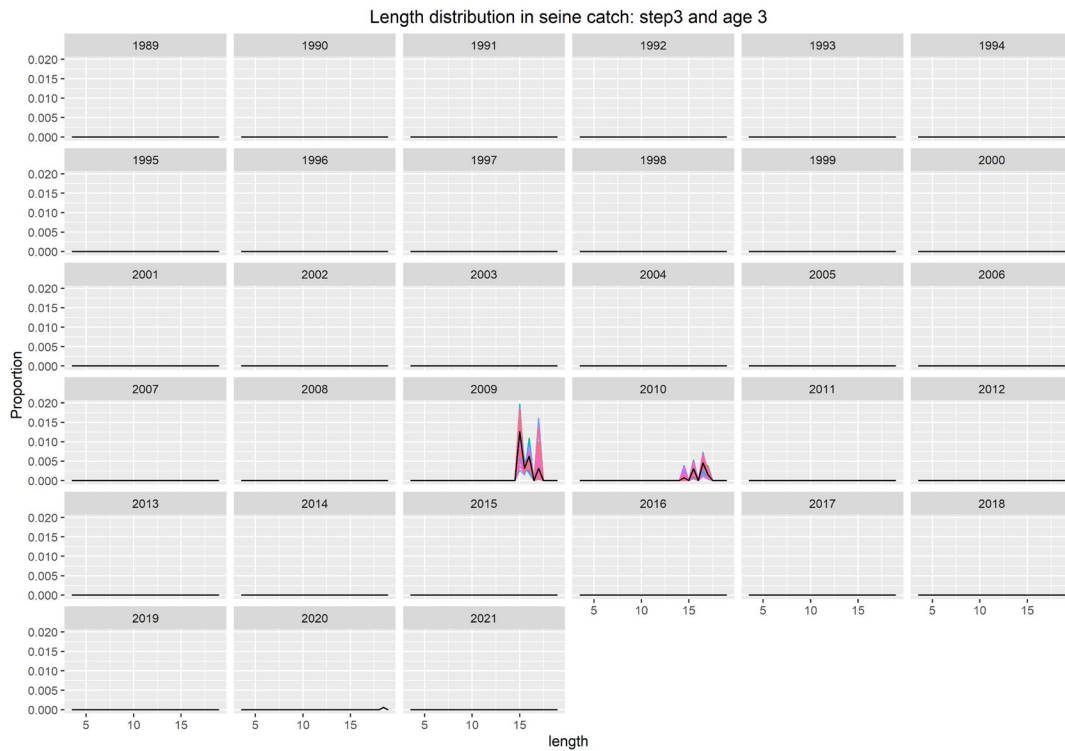
Figure 4.1.18.- One hundred parametric bootstrapped length distribution by year at age 3 and time-step 3 in the seine fleet (varied colors) compared to the original length distribution. In the commercial fleet, age-length distributions were obtained also in time steps 1, 2 and 4. The length distribution at age is presented only in time-step 3 because it has a good coverage for all the ages from 0 to 3 and is representative of what has been resampled in the other time steps.
