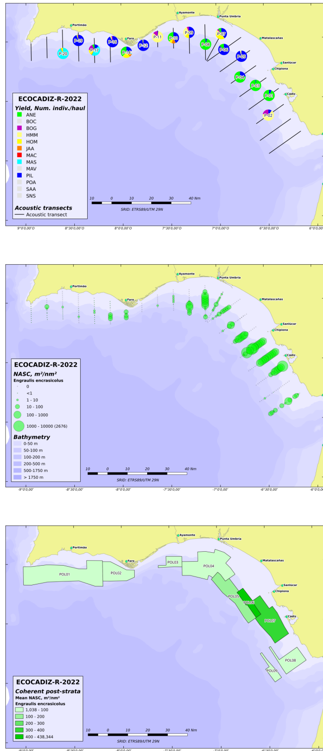
Figure 4.4.3.5. Anchovy in Division 9.a. Southern component. Subdivision 9.a South. ECOCADIZ-RECLUTAS 2022-10 survey (autumn Spanish acoustic survey in Subdivision 9.a South). Top: Location of valid fishing stations with indication of their species composition (percentages in number). Middle: Distribution of the backscattering energy (Nautical area scattering coefficient, NASC, in m 2 nm -2 ) attributed to the species. Bottom: distribution of homogeneous size-based post-strata used in the biomass/abundance estimates. Colour scale according to the mean value of the backscattering energy attributed to the species in each stratum.
