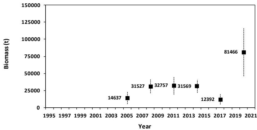
Figure 4.4.1.2. Anchovy in Division 9.a. Southern component. Subdivision 9.a South. BOCADEVA survey series (summer Spanish DEPM survey in Subdivision 9.a South). Series of SSB estimates ( \pm SD) obtained from the survey series.
