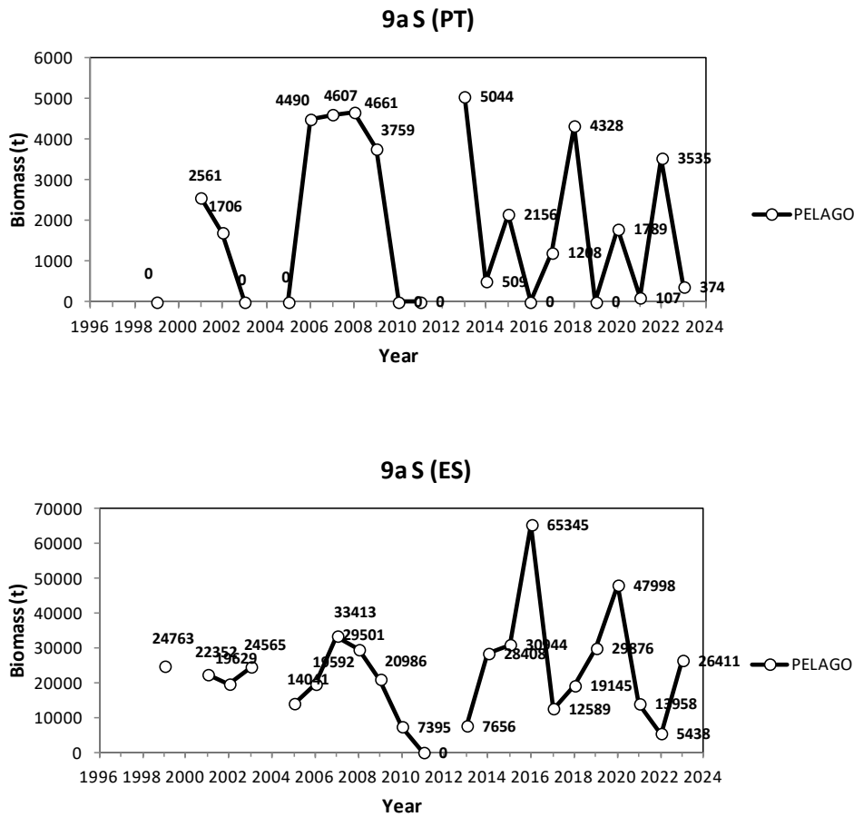
Figure 4.4.2.5. Continued. Acoustic estimates in the 9.a South differentiated by Portuguese (PT) and Spanish waters of the Gulf of Cadiz (ES). Note the different scale of the y-axis. Although estimates from Subdivision 9.a South in 2010 and 2014 were not separately provided for Algarve and Cadiz to this WG, the total estimated for the subdivision was assigned to the Cadiz area (by assuming some overestimation) according to the observed acoustic energy distribution in the area.
