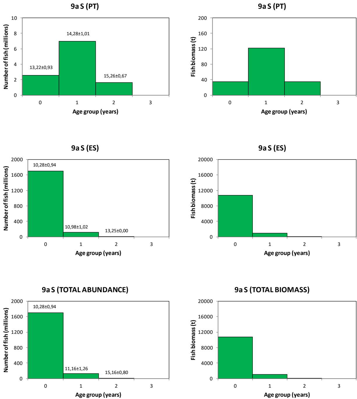
Figure 4.4.3.7. Anchovy in Division 9.a. Southern component. Subdivision 9.a South. ECOCADIZ-RECLUTAS 2022-10 survey (autumn Spanish acoustic survey in Subdivision 9.a South). Estimated abundances and biomasses (number of fish in millions and tonnes, respectively) for the surveyed area by age group, with indication of the mean size by age. Note the different scales in the y-axis.
