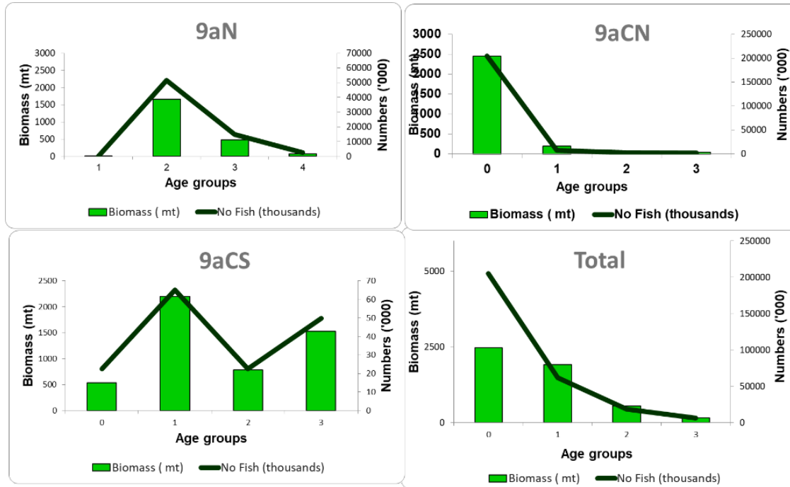
Figure 4.4.3.4. Anchovy in Division 9.a. Western component. Subdivisions 9.a North, 9.a Central-North and 9.a Central-South. IBERAS 0922 survey (autumn Spanish-Portuguese acoustic survey in Subdivisions 9.a North to Central-South). Estimated abundances and biomasses (number of fish in thousands and tonnes, respectively) for the surveyed area by age group, with indication of the mean size by age. Note the different scales in the y-axis.
