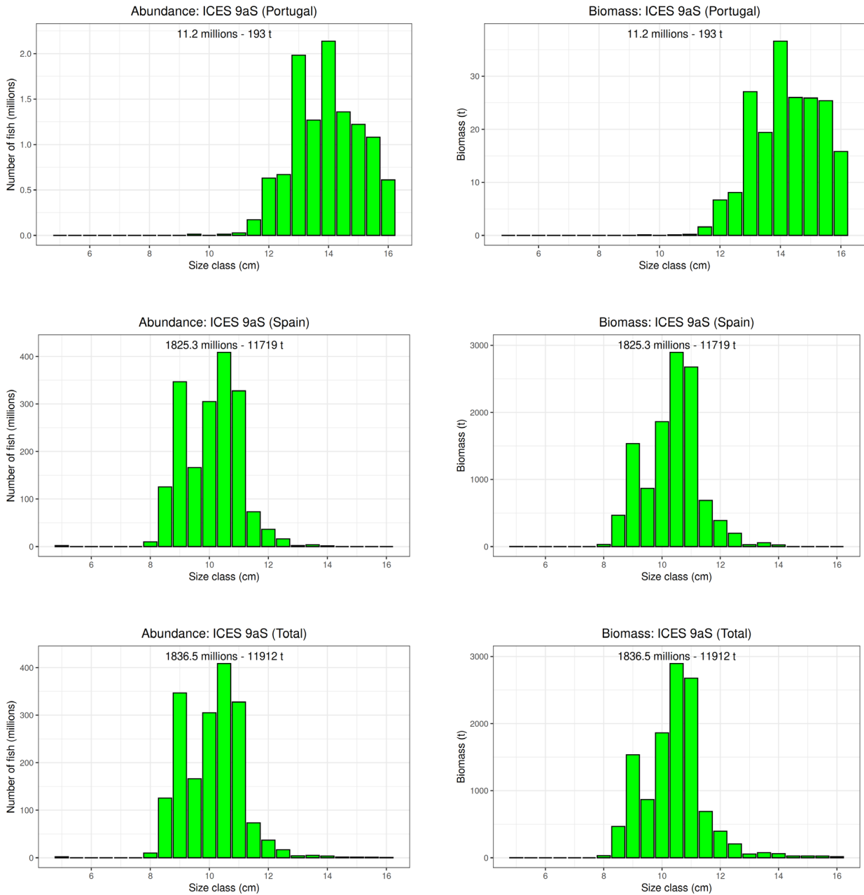
Figure 4.4.3.6. Anchovy in Division 9.a. Southern component. Subdivision 9.a South. ECOCADIZ-RECLUTAS 2022-10 survey (autumn Spanish acoustic survey in Subdivision 9.a South). Estimated abundances and biomasses (number of fish in millions and tonnes, respectively) for the surveyed area by length class (cm). Note the different scales in the y-axis.
