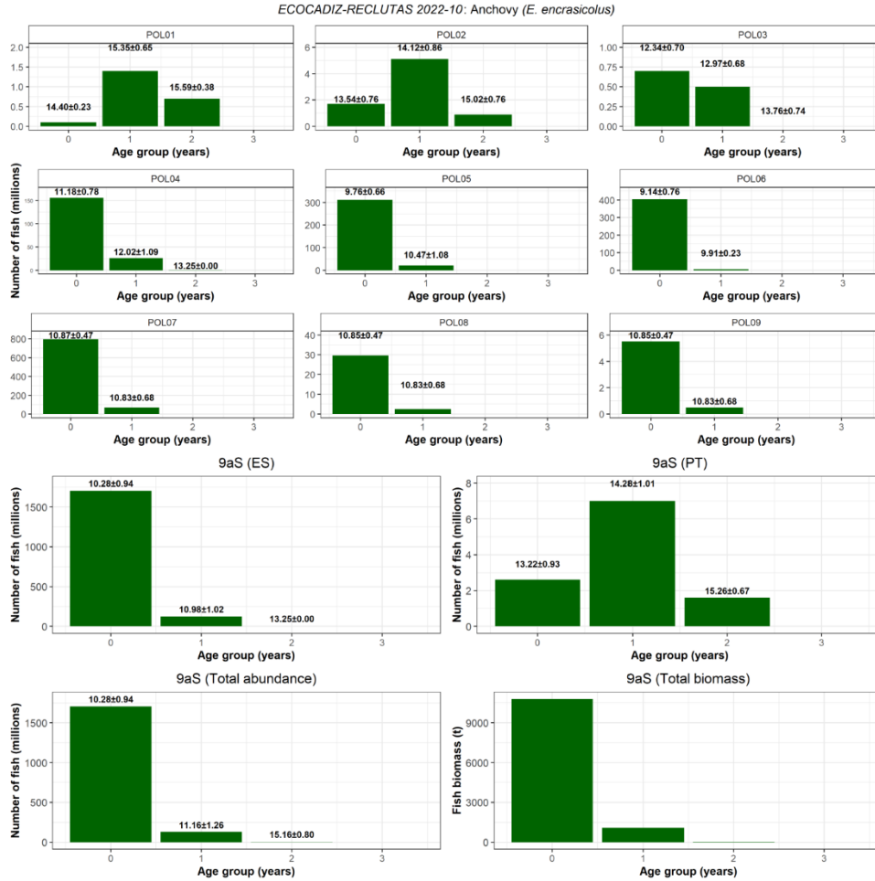
Figure 10. ECOCADIZ-RECLUTAS 2022-10 survey. Anchovy ( Engraulis encrasicolus ). Estimated abundances (number of fish in millions) by age group (years) by homogeneous post-stratum (POL01-POL09, numeration as in Figure 7 ) and total sampled area. Post-strata ordered in the W-E direction. Mean ( \pm SD) sizes of age groups are also shown. The estimated biomass (t) by age group for the whole sampled area is also shown for comparison. Note the different scales in the y axis.
