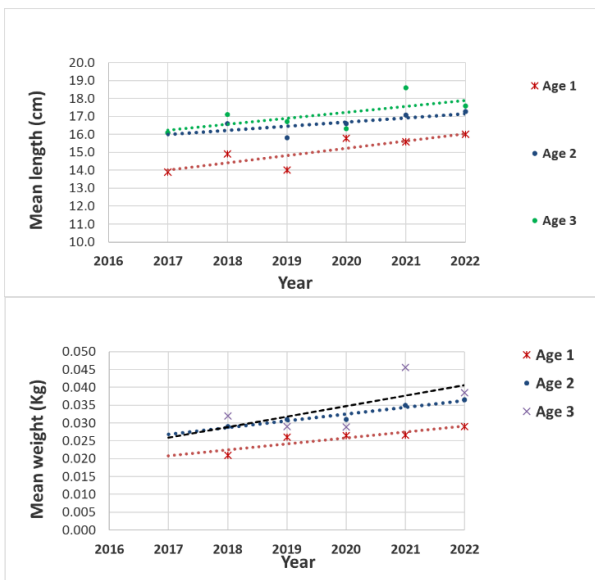
Figure 4.3.6.2. Anchovy in Division 9.a. Western component. Subdivision 9.a Central North. Portuguese fishery (all méti-ers). Cont'd. Annual mean length (TL, in cm) and weight (kg) at-age in the Portuguese catches of Western anchovy (2017 to 2022). Data for 2021 and 2022 are only available for the 3 rd and 4 th Quarters (represent 95% catches in 2021 and 70% catches in 2022).
