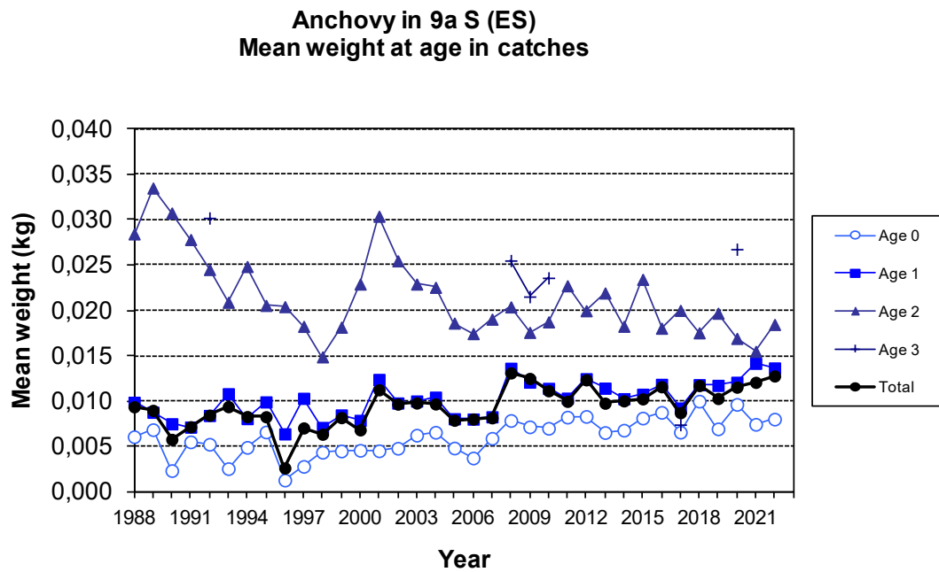
Figure 4.3.6.3. Anchovy in Division 9.a. Southern component. Subdivision 9.a-South. Spanish fishery (all métiers). Annual mean length (TL, in cm) and weight (kg) at-age in the Spanish catches of Gulf of Cadiz anchovy (1988–2022).
