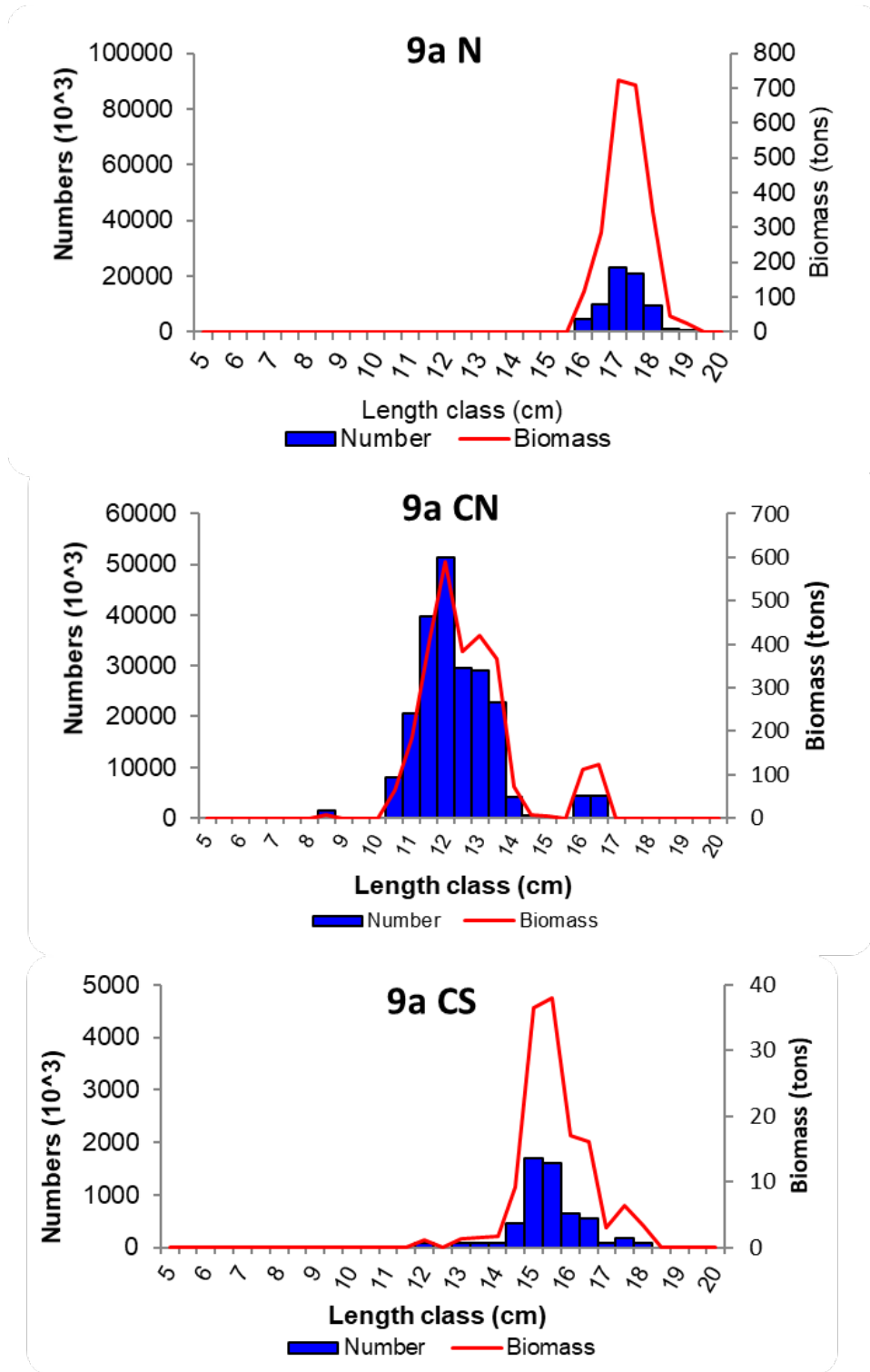
Figure 4.4.3.3. Anchovy in Division 9.a. Western component. Subdivisions 9.aNorth, 9.a Central-North and 9.a Central-South. IBERAS 0922 survey (autumn Spanish-Portuguese acoustic survey in Subdivisions 9.a North to Central-South). Estimated abundances and biomasses (number of fish in thousands and tonnes, respectively) for the surveyed area by length class (cm). Note the different scales in the y-axis.
