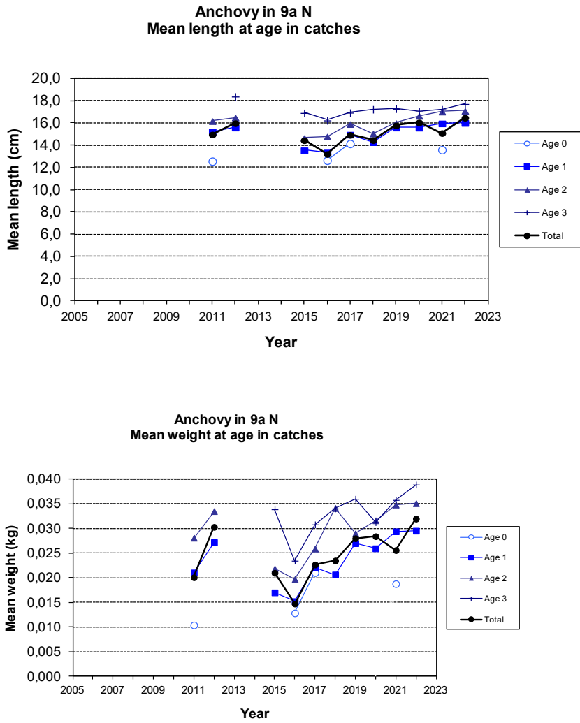
Figure 4.3.6.1. Anchovy in Division 9.a. Western component. Subdivision 9.a North. Spanish fishery (all métiers). Annual mean length (TL, in cm) and weight (kg) at-age in the Spanish catches of Western Galicia anchovy (2011–2022).
