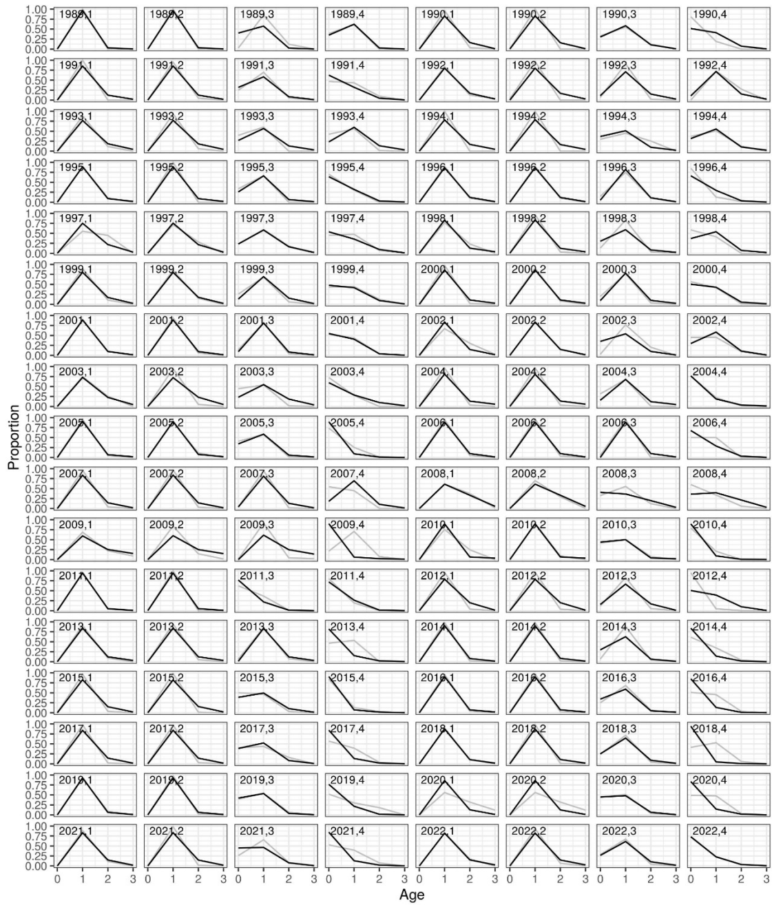
Figure 4.6.2.1.2.5. Anchovy in Division 9.a. Southern component. Comparison between observed and estimated quarterly catches age distribution from 1989 to 2022. Black lines represent estimated data while gray lines represent observed data. The number next to the year indicates the quarter.
