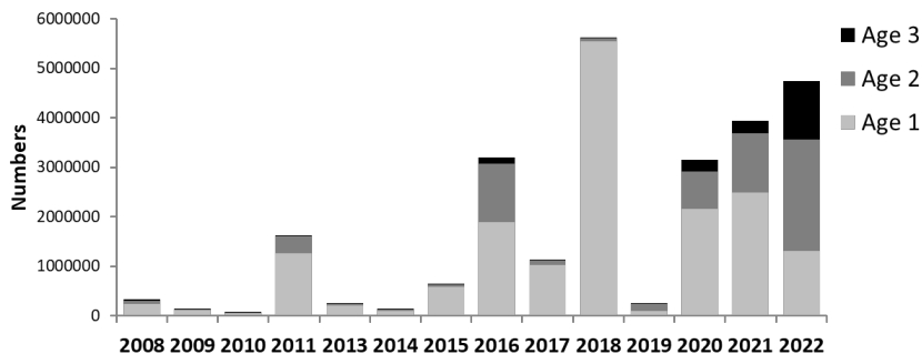
Figure 4.4.2.6. Anchovy in Division 9.a. Western component. Subdivisions 9.a North to Central-South. Annual trends of the estimated population by age class from the PELACUS (9a North) + PELAGO (9a Central-North and Central-South) Spring acoustic surveys. Age composition for 2020 only derived from the PELAGO survey given the PELACUS was not carried out. The age structure estimated for the PELACUS 0423 and PELAGO 23 survey has not been included in the figure because some inconsistencies were found in the age readings for the PELAGO 23 and age structure for the PELACUS 0423 is not yet available.
