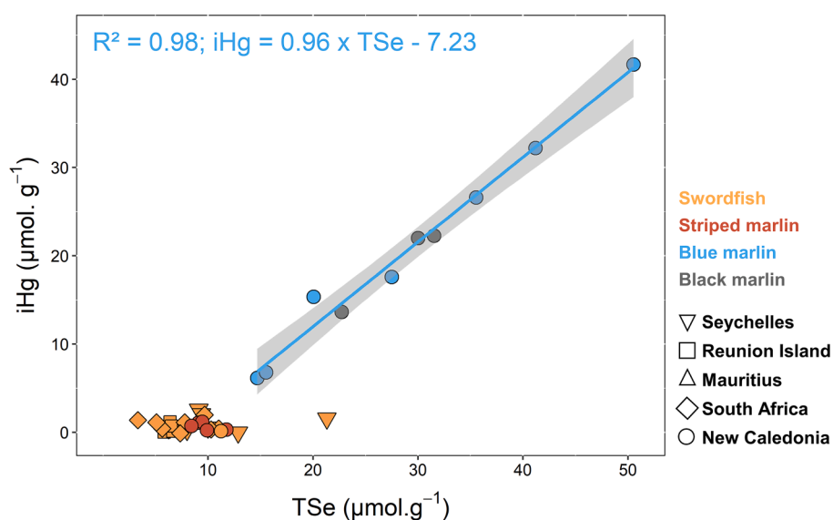
Fig. 4. Relationship between inorganic mercury (iHg) and total selenium (TSe) molar concentrations ( \mu\text{mol}\cdot\text{g}^{-1} ) in billfish muscle samples. Colours and shapes of the symbols refer to species and samples provenance, respectively. The blue line and the grey shadow represent the significant linear regression between the two variables found for blue marlin only ( p < 0.05 ; p > 0.05 for striped marlin and swordfish; not tested for black marlin because of insufficient sample availability), and the standard deviation, respectively. (For interpretation of the references to colour in this figure legend, the reader is referred to the web version of this article.)
