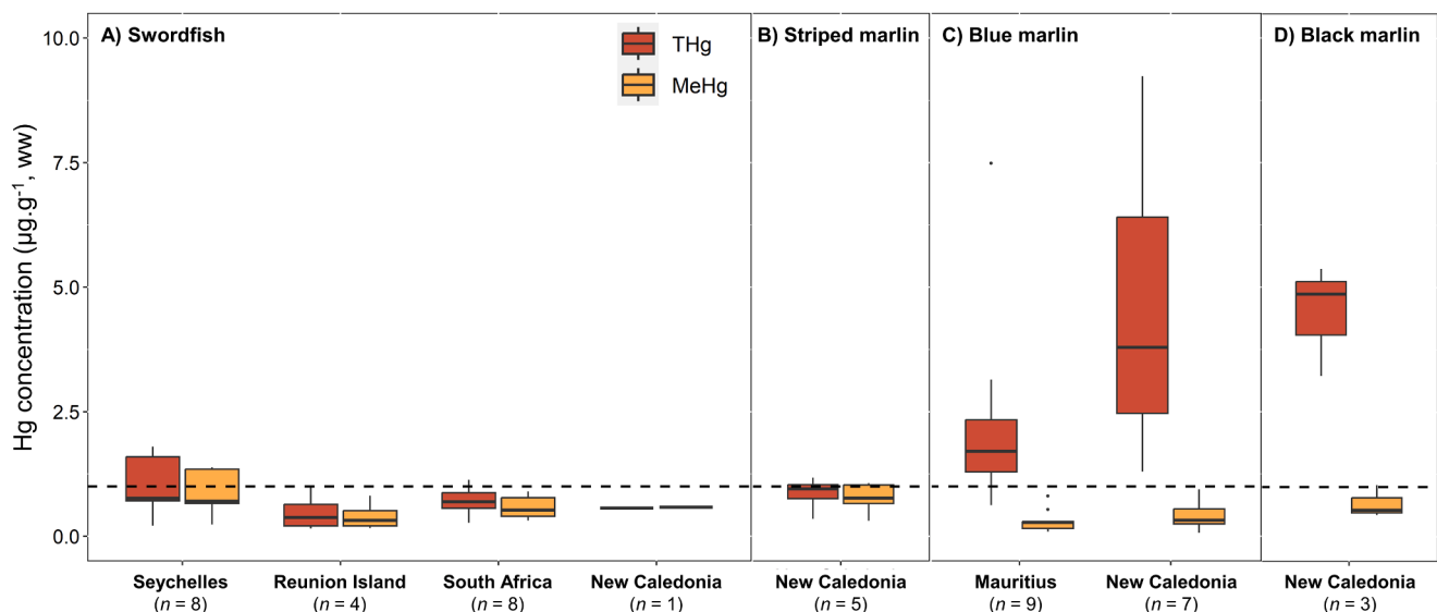
Fig. 2. Variability of mercury content in billfish muscle. Boxplots of total mercury (THg) and methylmercury (MeHg) concentrations ( \mu\text{g}\cdot\text{g}^{-1} , ww) in muscle samples of A) swordfish, B) striped marlin, C) blue marlin, and D) black marlin, caught in different regions of the Indian (i.e., Seychelles, Reunion Island, South Africa, and Mauritius) and the Pacific (i.e., New Caledonia). The dashed line represents the MeHg consumption guideline value for large predatory fish of 1 \mu\text{g}\cdot\text{g}^{-1} ww (FAO and WHO, 2005)(FAO Codex Alimentarius Commission, 2019). (For interpretation of the references to colour in this figure legend, the reader is referred to the web version of this article.)
