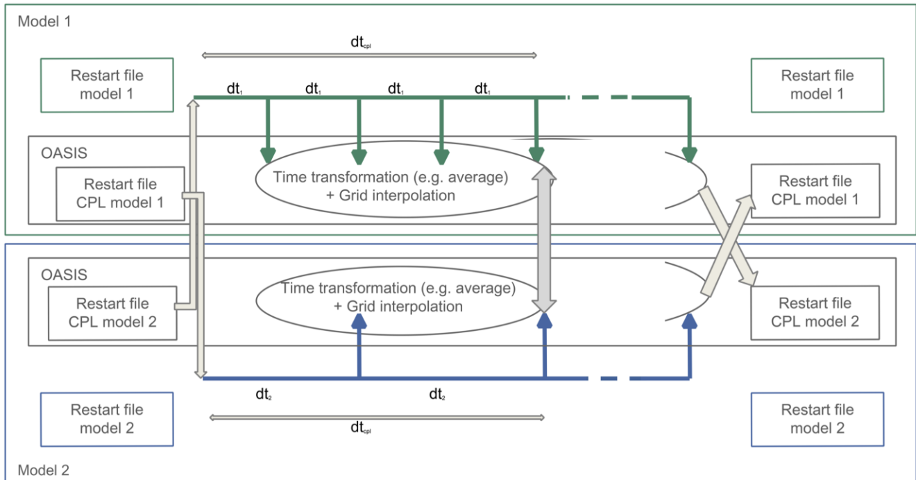
170 Figure 3: Schematic view of the coupling sequence used in a coupled simulation between 2 models interfaced using the OASIS3-MCT library.
