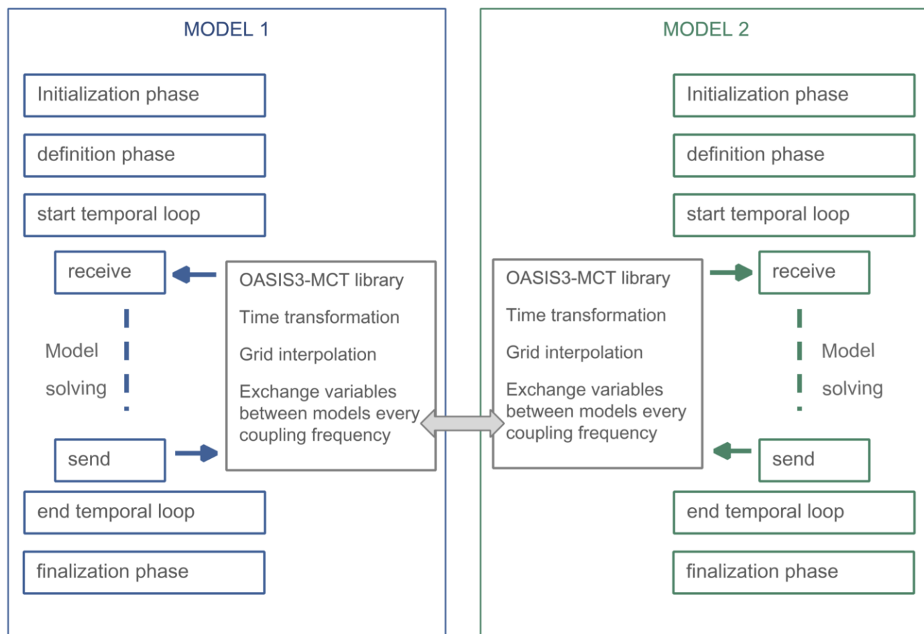
Figure 2: Schematic view of the coupling steps implemented in WRF coupling interface: initialization, definition, exchanges, finalization. Here is an example of 2 models coupled through OASIS3-MCT is illustrated.
