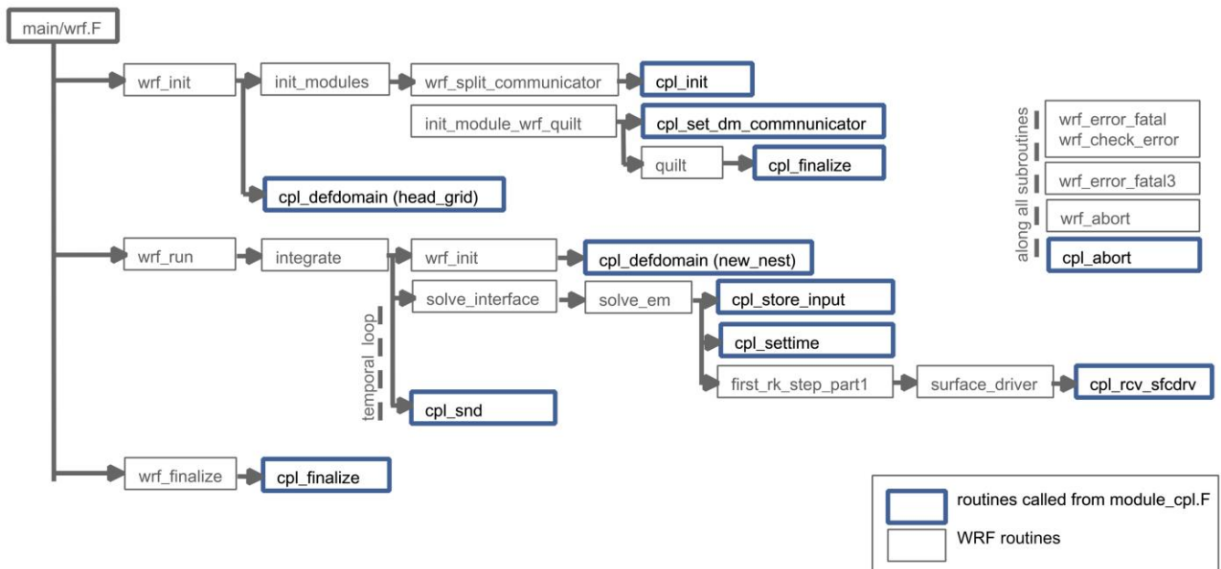
220 Figure 4: Schematic view of the coupling interface implementation in WRF. WRF original routines are in grey. All new routines (in blue) are gathered in “frame/module_cpl.F”.
