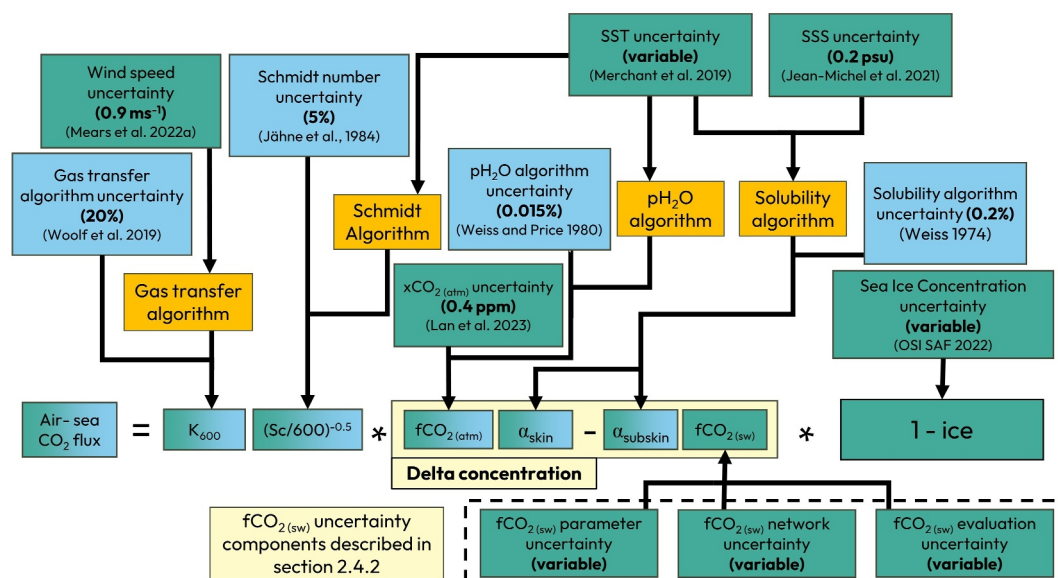
Figure 1. Flowchart indicating the sources of uncertainty ( 2\sigma ) that contribute to each term in the air-sea CO 2 flux calculation described in Section 2.2 and integrated in Section 2.5. Green boxes indicate a component that decorrelates over a spatial and temporal scale, blue boxes indicate globally correlated components and orange boxes indicate functions for which uncertainties are propagated using a Monte Carlo approach. Boxes with a green to blue gradient indicate that the component has both globally correlated, and spatially correlated components. The f\text{CO}_2(\text{sw}) uncertainty components (grouped by the dashed line box) are described in Section 2.4.2. References within the flowchart are for the gas transfer algorithm uncertainty (Woolf et al., 2019), wind speed uncertainty (Mears et al., 2022a), Schmidt number algorithm uncertainty (Jähne et al., 1984), partial pressure of water vapor (pH 2 O) algorithm (Weiss & Price, 1980), xCO 2 (atm) uncertainty (Lan et al., 2023), SST uncertainty (Merchant et al., 2019), SSS uncertainty (Jean-Michel et al., 2021), solubility algorithm uncertainty (Weiss, 1974) and the sea ice concentration uncertainty (OSI SAF, 2022). Acronyms in the flowchart are gas transfer coefficient ( K_{600} ), Schmidt number (Sc), fugacity of CO 2 in atmosphere ( f\text{CO}_2(\text{atm}) ) and seawater ( f\text{CO}_2(\text{sw}) ) and solubility at the subskin ( \alpha_{\text{subskin}} ) and skin ( \alpha_{\text{skin}} ).
