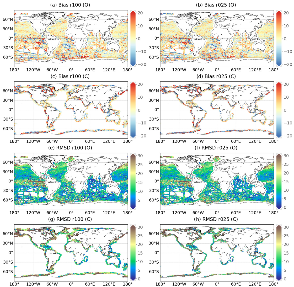
Figure A3. Global maps of mean model–data difference (bias, a–d ) and root-mean-square deviation (RMSD; e–h ) between the reconstruction and SOCATv2022 p\text{CO}_2 ( \mu\text{ atm} ) over 1985–2021. ( a, c, e, g ) CMEM-LSCE-FFNN with a resolution of 1^\circ (r100); ( b, d, f, h ) CMEM-LSCE-FFNN with a resolution of 0.25^\circ (r025). Open-ocean data (O) in each 0.25^\circ grid box used for evaluation are created by setting conservatively the open-ocean SOCATv2022 data value at the 1^\circ grid box containing it. Coastal-ocean data (C) are extracted from each of the two SOCATv2022 gridded data products.
