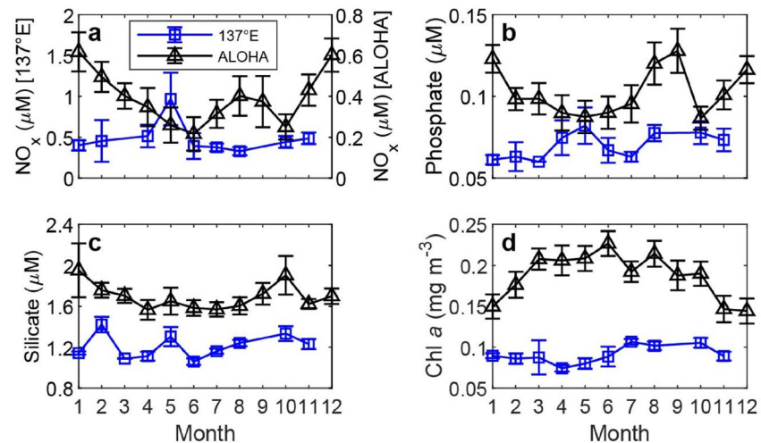
Figure 11. Subsurface isopycnal monthly mean climatology of biogeochemical properties along 137°E and at Station ALOHA in the North Pacific Subtropical Gyre (NPSG), including concentrations of (a) NO x , (b) phosphate, (c) silicate, and (d) Chl a . Isopycnal layers with potential densities ( \sigma_\theta ) of 23.0 and 24.5 kg m -3 were selected for 137°E and Station ALOHA, respectively, to represent the deep chlorophyll maximum layer. The data at 137°E are from the Global Ocean Data Analysis Project v2.2022 product (Lauvset et al., 2022) ( https://www.glopad.info/index.php/merged-and-adjusted-data-product-v2-2022/ ) in the NPSG center (10°–20°N). The data at Station ALOHA are from Hawaii Ocean Times-series ( https://hahana.soest.hawaii.edu/hot/hot-dogs/ ), in which the low-level concentrations of NO x and phosphate measured by highly sensitive methods are used. Note that the concentrations of NO x along 137°E and at Station ALOHA are plotted using different scales. Chl- a concentrations at Station ALOHA were measured by high-performance liquid chromatography.
