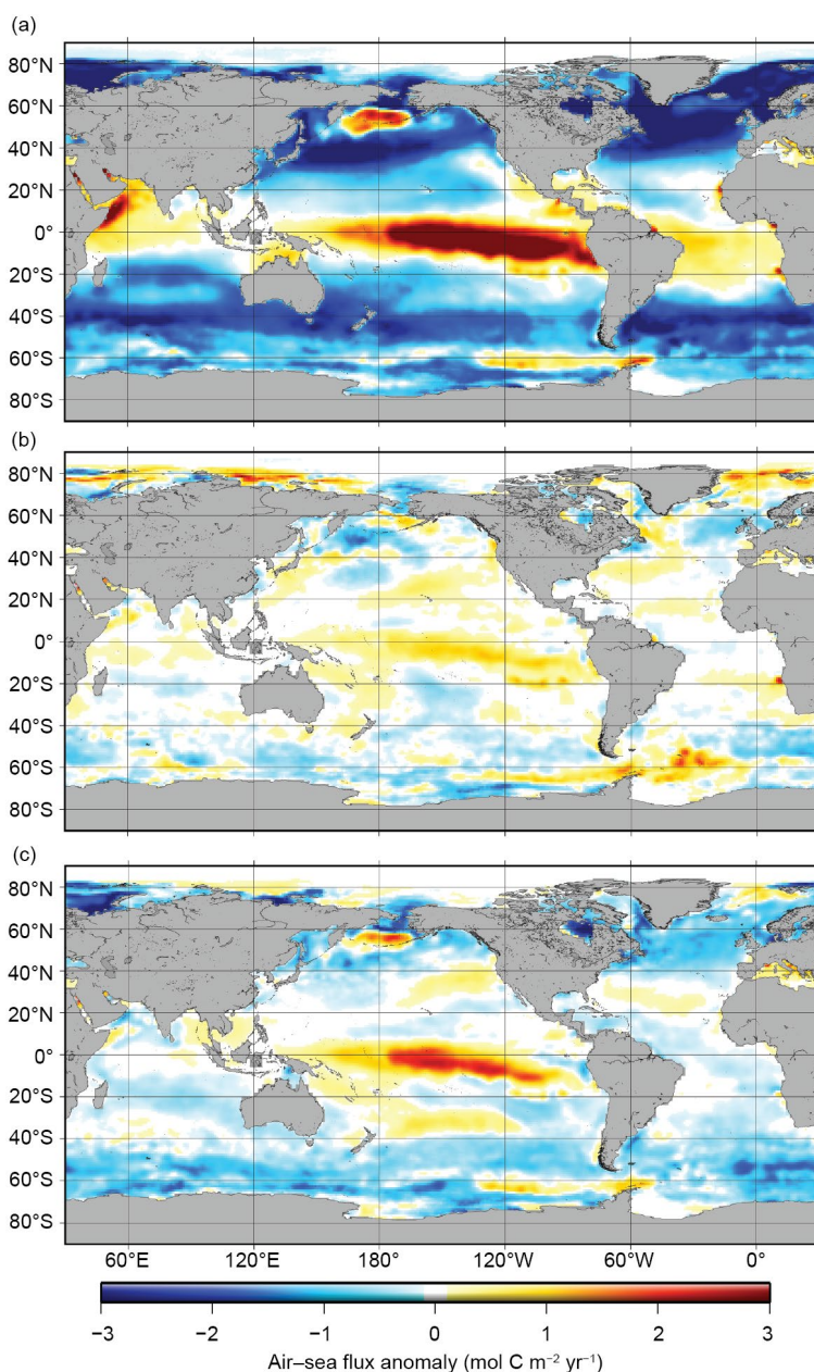
Fig. 3.29. Global map of (a) net air-sea carbon dioxide (CO 2 ) fluxes for 2022, (b) net air-sea CO 2 flux anomalies for 2022 minus 2021, and (c) net air-sea CO 2 flux anomalies for 2022 relative to 1990–2020 average values using the SOM-FNN approach of Landschützer et al. (2013). Units are all mol C m -2 yr -1 . Ocean CO 2 uptake regions shown in the blue colors.
