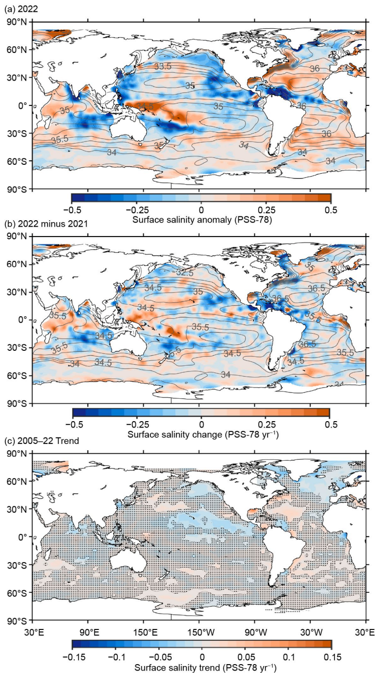
Fig. 3.7. (a) Map of the 2022 annual sea-surface salinity anomaly (colors, Practical Salinity Scale-78 [PSS-78]) with respect to monthly climatological 1955–2012 salinity fields from WOA13v2 (yearly average; gray contours at 0.5 intervals, PSS-78). (b) Difference of 2022 and 2021 sea-surface salinity maps (colors, PSS-78 yr -1 ). White ocean areas are too data-poor (retaining <80% of a large-scale signal) to map. (c) Map of local linear trends estimated from annual sea-surface salinity anomalies for 2005–22 (colors, PSS-78 yr -1 ). Areas with statistically insignificant trends at 5%–95% confidence are stippled. All maps are made using Argo data.
