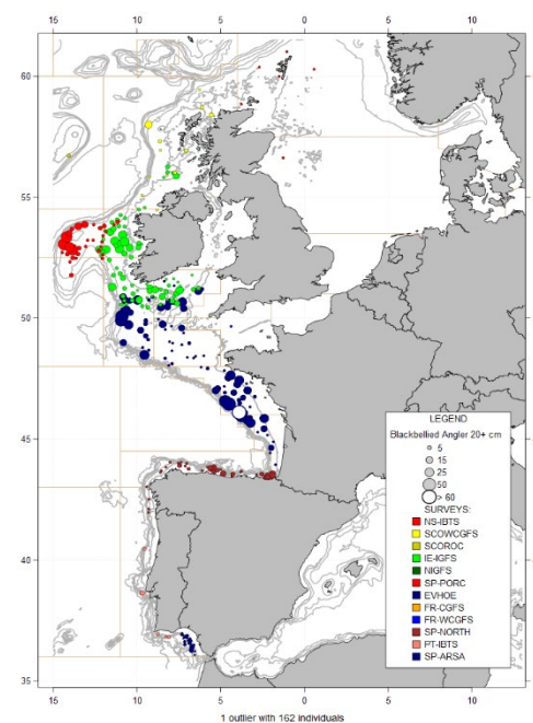
Figure A.8.21. Catches in numbers per hour of 1+ group black-bellied anglerfish, Lophius budegassa ( \geq 20 cm), in summer/autumn 2023 IBTSurveys.
