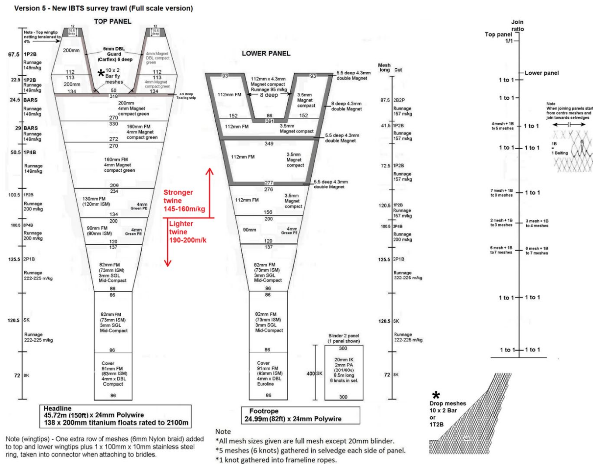
Figure 4.1. Net plan for the developed survey trawl (full-scale version). Version 5 of 17 May 2024.
