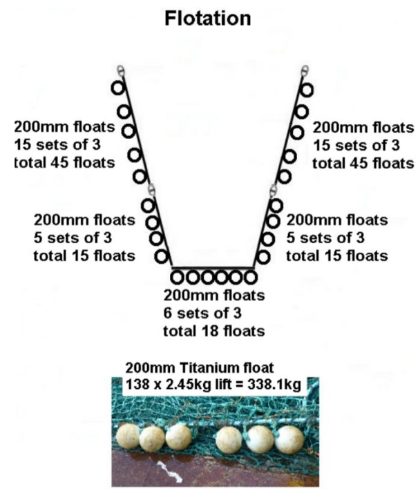
Figure 4.5. Current flotation specification, including positioning around the headline, for the developed survey trawl (full-scale version). Version 5 of 17 May 2024.
