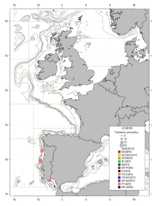
Figure A.8.43. Catches in numbers per hour per hour of blue jack mackerel, Trachurus picturatus , in summer/autumn 2023 IBTSurveys.
