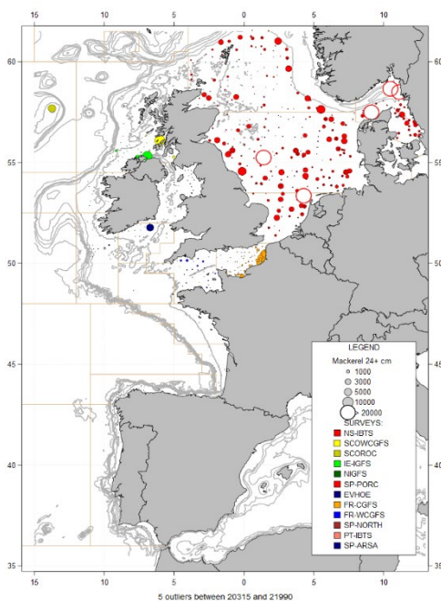
Figure A.8.13. Catches in numbers per hour of 1+ group mackerel, Scomber scombrus (≥24 cm), in summer/autumn 2023 IBTSurveys.
