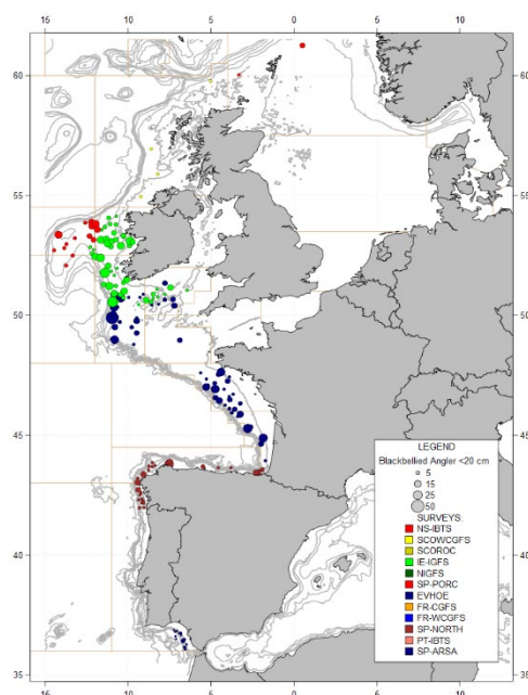
Figure A.8.20. Catches in numbers per hour of 0-group black-bellied anglerfish, Lophius budegassa (<20 cm), in summer/autumn 2023 IBTSurveys.
