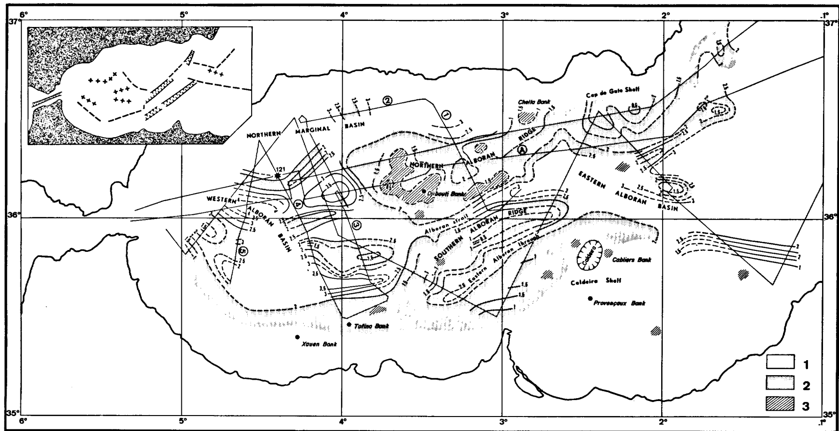
Figure 2. Topographic map of the acoustic basement. Basement isochrons are in second d.t. from the water surface. Numbers 1 to 5 give the position of the Jean Charcot seismic profiles presented here. A. is the Glomar Challenger profile. Dashed-lines: substratum higher than 2.5 sec. d.t. Stippled lines: probably vulcanites. Black dots are the position of the dredge hauls (Giermann et al.).
