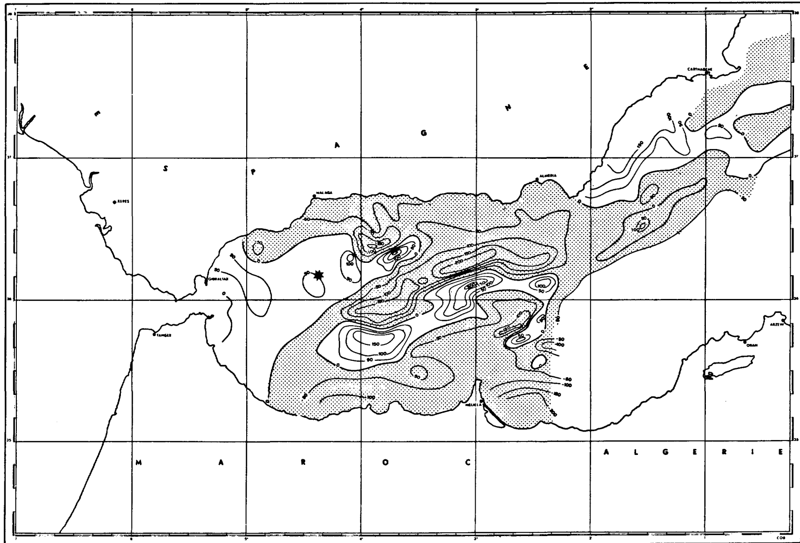
Figure 10. Map of the residual magnetic field in the Alboran sea (after Vogt et al., 1971). Contour interval is 50 gammas.
