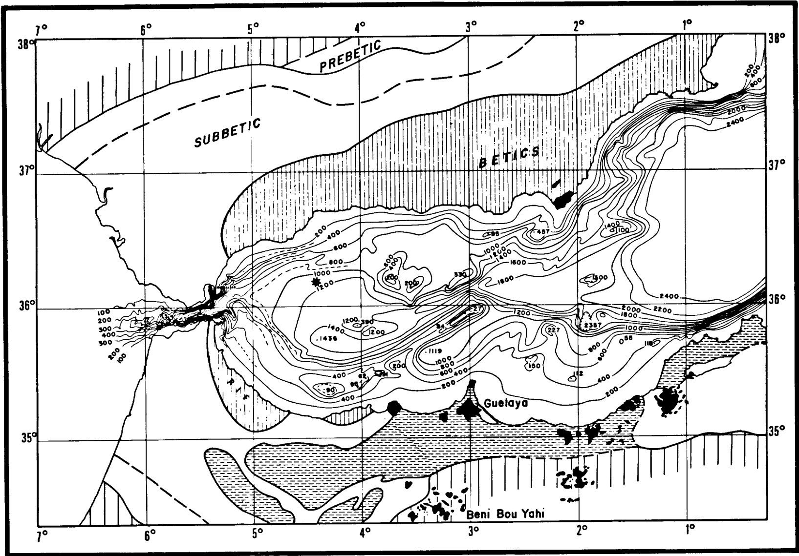
Figure 1. Bathymetric map of the Alboran Basin (Ryan, Giermann, Vogt, as modified by S. Monti), and schematic structural features. (1) Rif and Betics: internal zones; (2) zone of gliding nappes; (3) external zone (autochthonous and semi-autochthonous); (5) volcanites.
