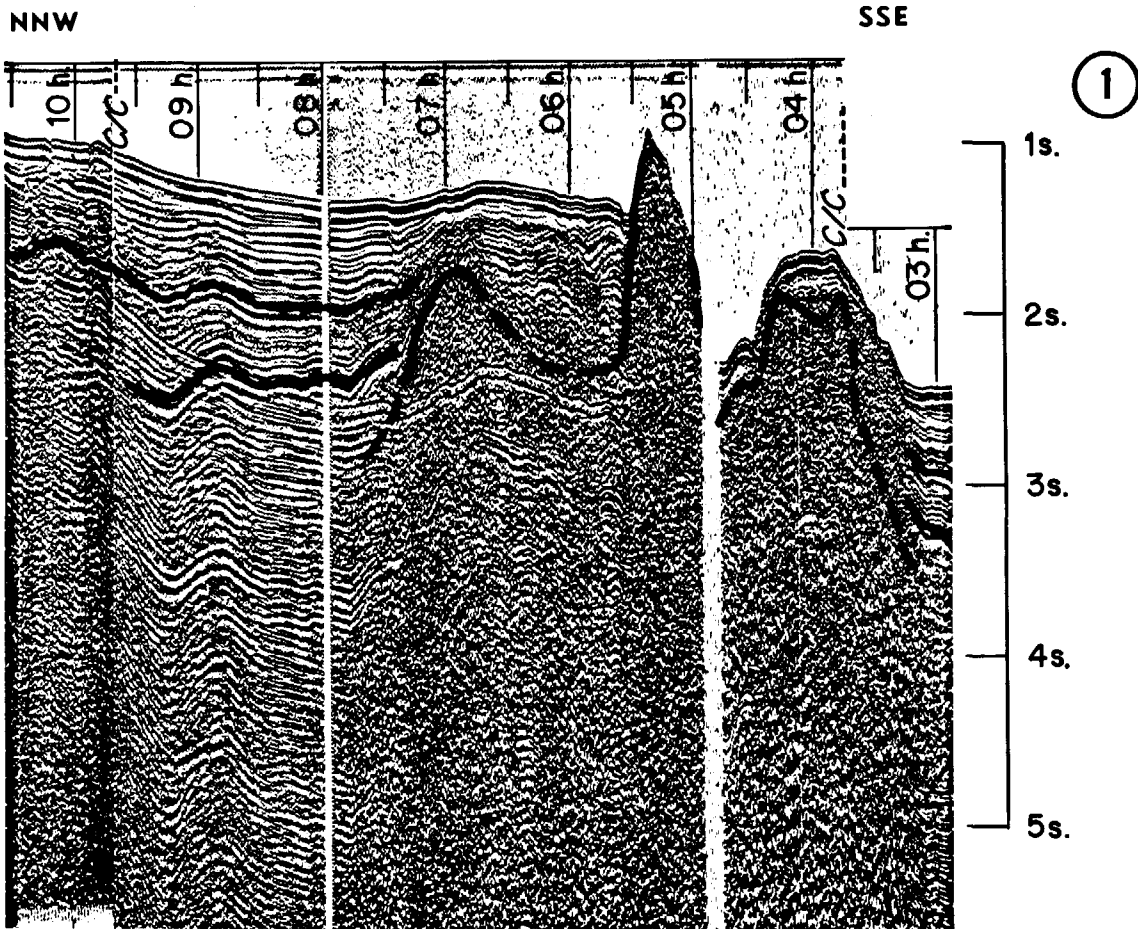
Figure 3. Flexotir profile No. 1 on the Alboran shoal and on the northern marginal basin. Note the important seamount (probably volcanic) in the northern part of the Alboran Strait. The two underlined reflectors in the sedimentary cover are probably the base of the Pliocene and the Quaternary.
