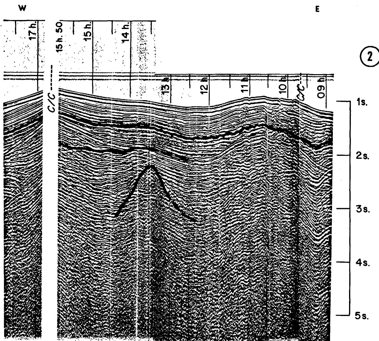
Figure 5. Profile 2 (Flexotir Jean Charcot). This profile is on the northern marginal basin. Note the relief of the basement in the middle of the basin. Underlined reflectors may represent the possible base of the Pliocene and the Quaternary.
