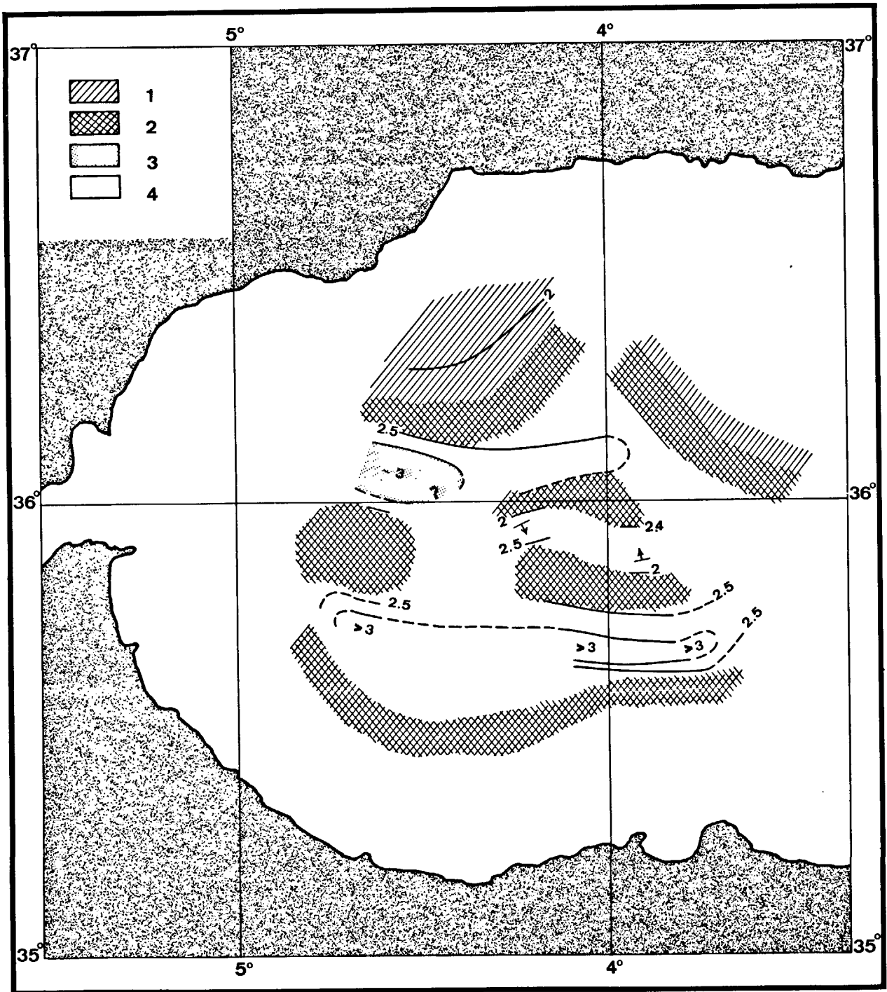
Figure 9. Messinian surface isochrons (d.t.): (1) area with erosion surface (Messinain); (2) area where the substratum is covered by thin prepliocene sediments or no prepliocene sediments; (3) possible evaporitic basin; (4) folded area.
