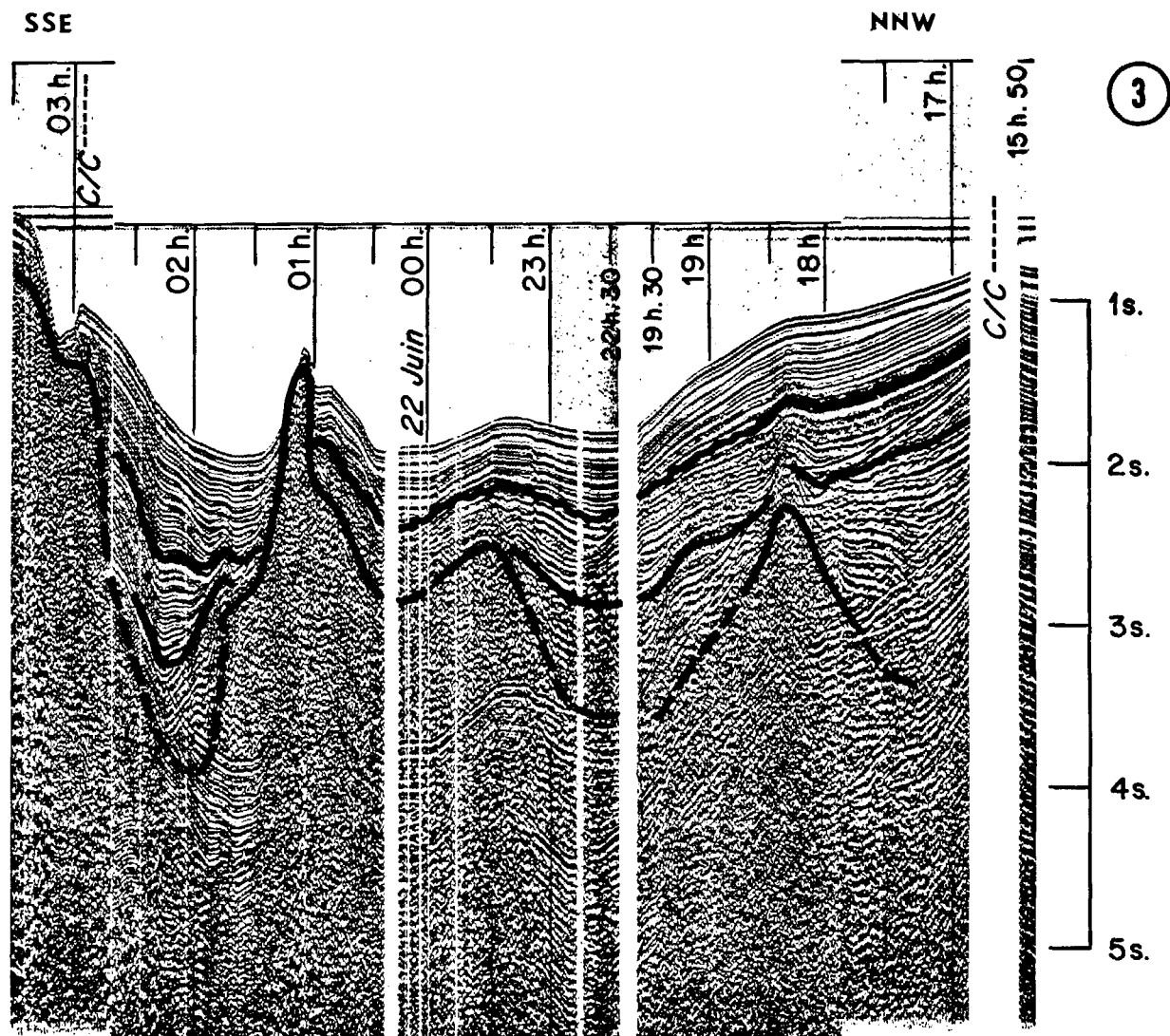
Figure 6. Profile 3 (Flexotir Jean Charcot). Substratum, possible base of the Pliocene and the Quaternary are underlined. One can see the Messinian erosion surface in the northern part.
