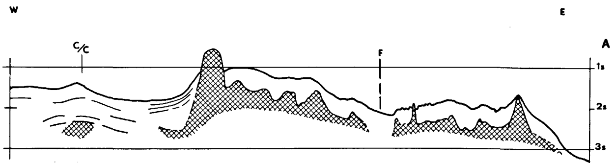
Figure 4. Profile A Glomar Challenger (profile with air-gun). It is possible to follow the substratum on the northern Alboran Ridge and the Cap of Gate shelf. Note the two volcanic seamounts limiting the shoals.
