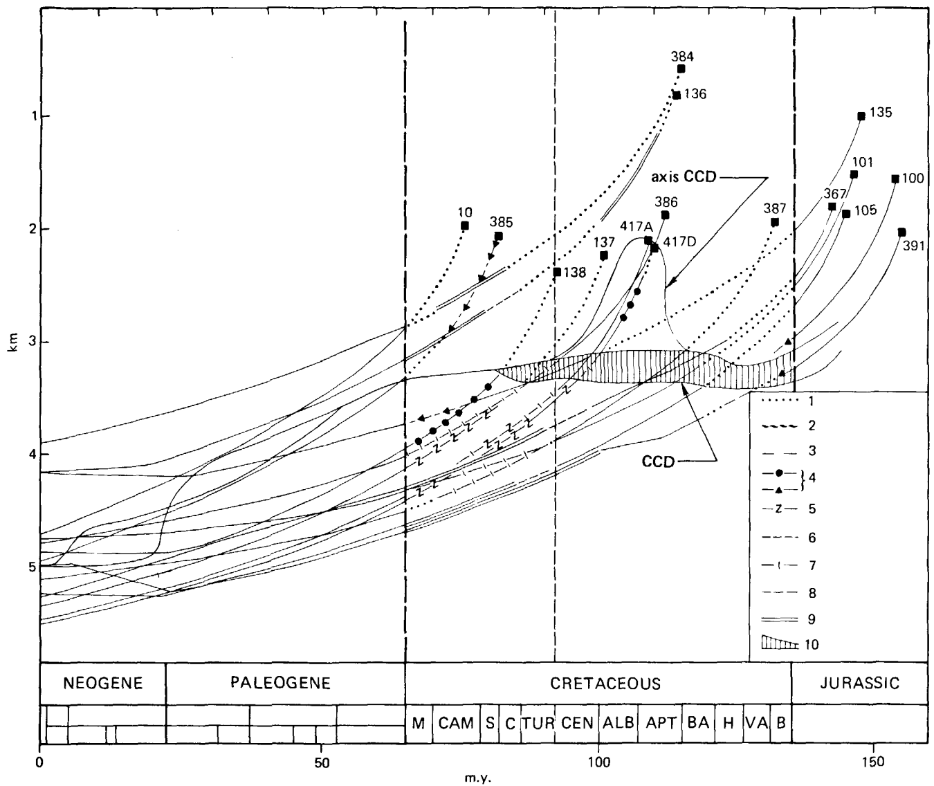
Figure 5. Subsidence curves of Central Atlantic sites emphasizing facies distribution in the Cretaceous. Key to symbols is the same as in Figure 4.
