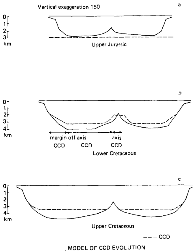
Figure 10. Model of CCD evolution at three different periods. The CCD level is marked by a dashed line. The Lower Cretaceous diagrammatic section shows the postulated axis CCD.
