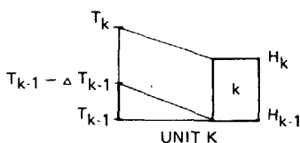
Figure 2. Depth-time treatment of a drill site. The density of sedimentary unit is d_k .
