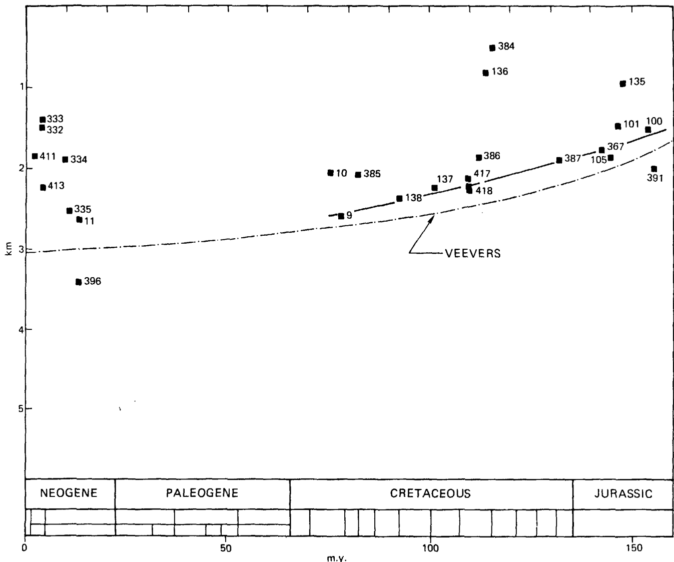
Figure 6. Subsidence curves of Central Atlantic sites emphasizing evolution of facies distribution in the Cenozoic. Key to symbols is the same as in Figure 4.
