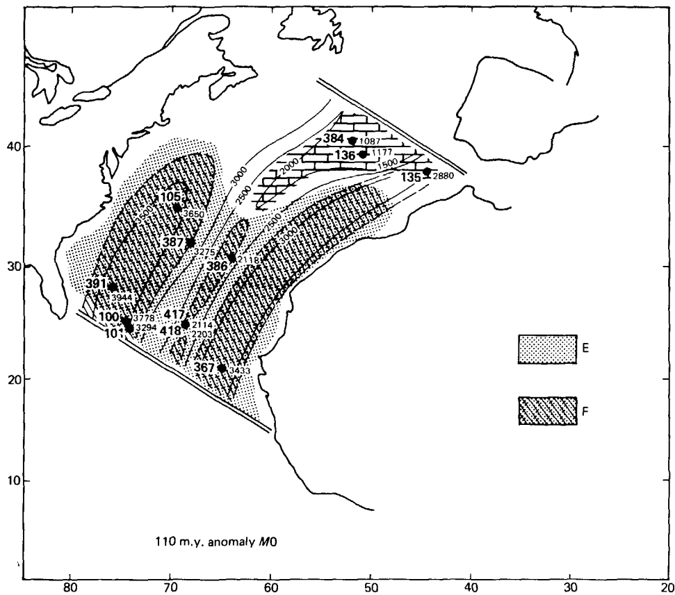
Figure 7. Bathymetric and geographic map for magnetic anomaly MO time (110 m.y.). The black dots mark the position of the site. The number to the right is the depth. E: black shales (Facies 3); F: carbonate-free black shales. The chalk pattern indicates limestone (Facies 1). The rotation applied to Africa and its sites is 65^{\circ}.6N\ 20^{\circ}.2W ( -55^{\circ} ). North America and its sites are held fixed. The Newfoundland and Guinea-Bahama fracture zones are shown by parallel lines.
