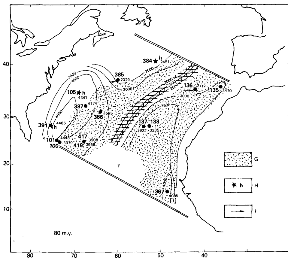
Figure 8. Bathymetric and geographic map for magnetic anomaly 34 time (80 m.y.). G: Undifferentiated clays including zeolitic clay (Facies 5), radiolarian clay (Facies 4), and multicolor clay (Facies 7); H: hiatus; I: reworked sediments (silt, turbidites) (Facies 8). A carbonate belt has been placed along the axis of the Mid-Atlantic Ridge. The rotation applied to Africa is 79^{\circ}.1N , 15^{\circ}.7W ( -30.4^{\circ} ). North America is held fixed.
