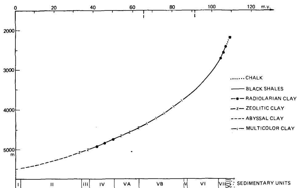
Figure 3. Subsidence curve for Hole 417D, illustrating the depths of deposition of each sediment unit. The black square represents the initial depth at the ridge crest when the site was created.
