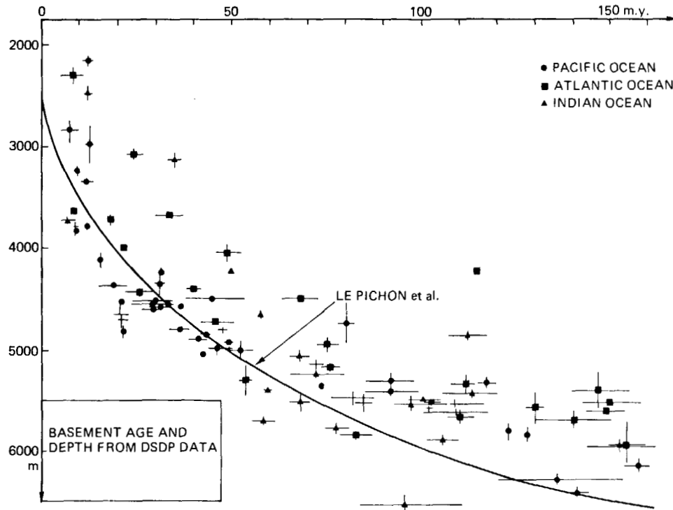
Figure 1. Basement age and depth from deep-sea drilling data. The range in observed depths to basement and absolute ages inferred from fossil evidence are indicated by vertical and horizontal bars, respectively. The curve drawn through the data points is the empirical exponential fit of Le Pichon et al. (1973) and does not match well the depth flattening occurring around 80 m.y.
