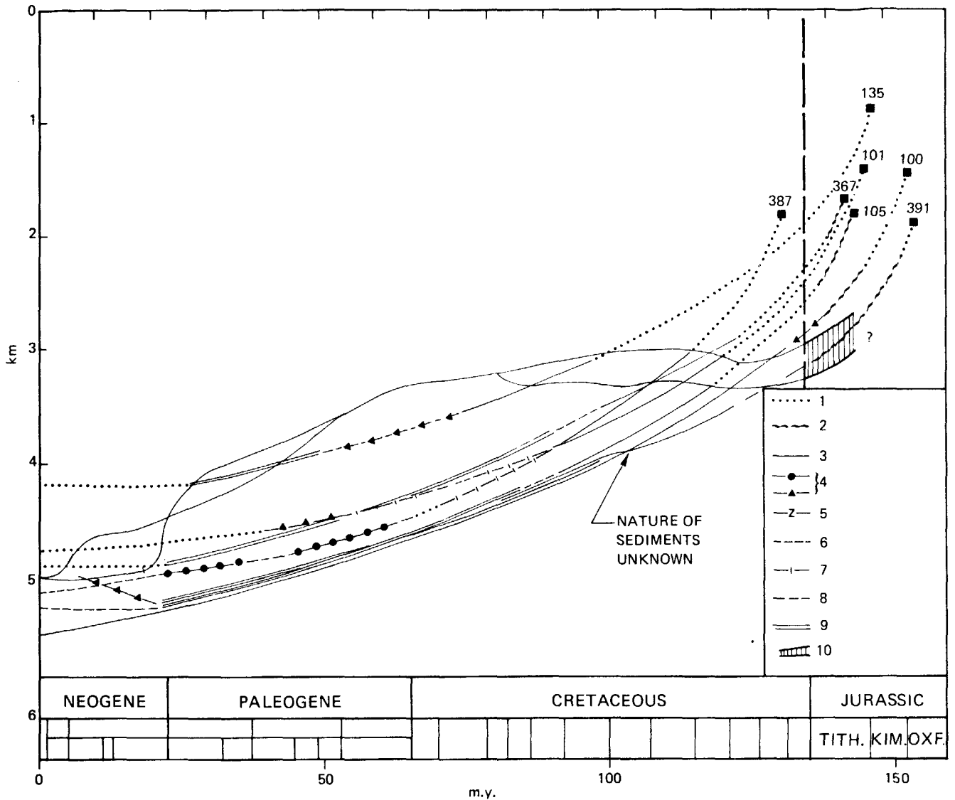
Figure 4. Subsidence curves of central Atlantic sites emphasizing Jurassic sites. 1: limestone; 2: red clayey limestone; 3: black shales; 4: radiolarian clay and cherty clay; 5: zeolitic clay; 6: abyssal clay; 7: multicolor clay; 8: redeposited sediments; 9: hiatus; 10: range of CCD levels. The black square with site number is the crestal depth.
