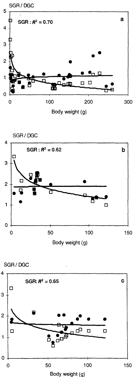
Figure 2. Relationship between body weight (BW) and two growth descriptors (SGR = specific growth rate (●); DGC = daily growth coefficient (□)) in (a) seabass, (b) seabream and (c) turbot. Based on data from personal experimental work as well as from the literature.
