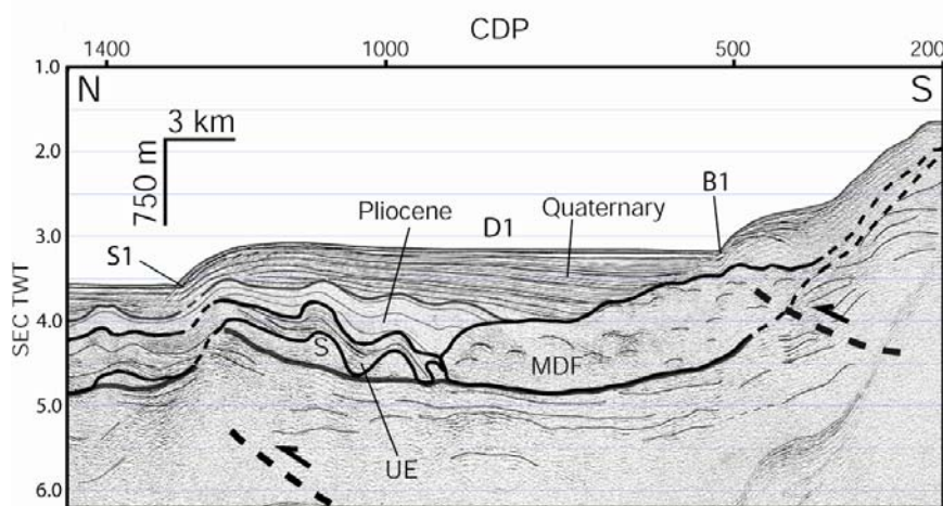
Figure 2. Time-migrated, stacked 6-channel seismic line A and its interpretative cross section showing cumulative wedge and progressive unconformity in the deep basin (see Figure 1 for location). S: salt; MDF: Messinian detritic fan; UE: Upper Evaporites (roof at ~5.3 Ma). S1 and B1 are scarps (Figure 1). Heavy dashed lines are thrust ramps inferred. Note that the UE layer has a roughly constant thickness, indicating that it predates tectonic activity.
