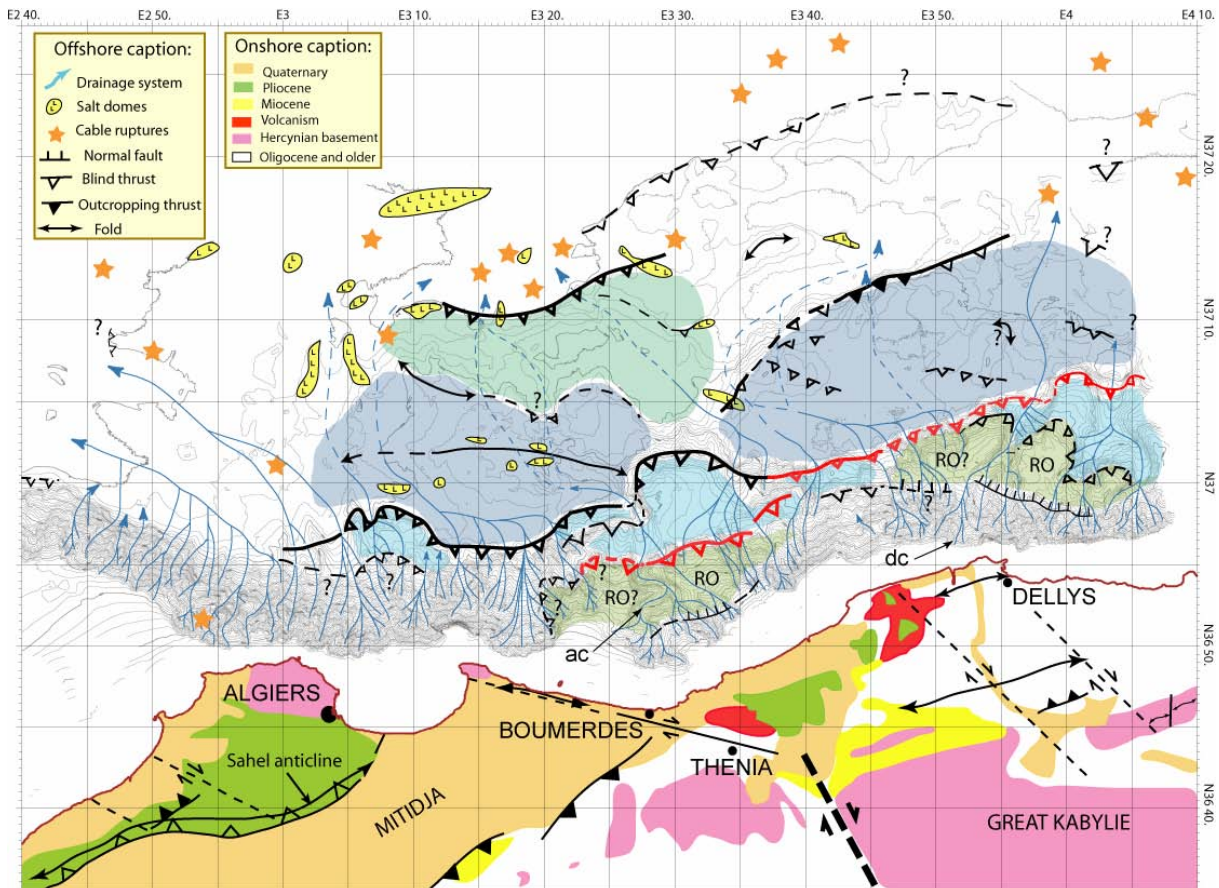
Figure 4. Tectonic map interpreted from data analysed in this study. Onland geology modified from Boudiaf et al. [1998] and Ayadi et al. [2003]. Red line is the proposed prolongation of the 2003 rupture determined by Delouis et al. [2004] to the seafloor, depicting two main segments [B1 and B2, Figure 1). RO: Rollover basin. Coloured areas off RO are piggyback basins. Bathymetry is shaded.
