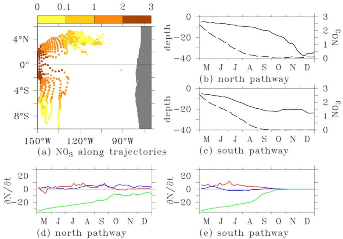
Fig. 6a-e Results of the direct experiment: drifters are released at 150°W in May 1997 and reach their end point in December 1997. a Evolution of the nitrate concentration (μM; color key) along the trajectories. b Time-series of the mean depth (m; solid line ) and NO 3 concentration (μM; dashed line ) along the northern pathway. c Time-series of the mean depth and NO 3 concentration along the southern pathway. d Time-series of the horizontal diffusion ( blue line ), vertical diffusion ( red line ) and biological uptake ( green line ) in μmol NO 3 m -3 d -1 along the northern pathway. e Time-series of the horizontal diffusion, vertical diffusion and biological uptake along the southern pathway.
