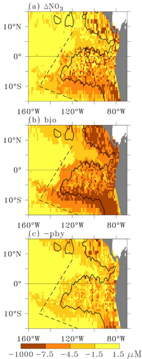
Fig. 7a-c Maps of the (a) \text{NO}_3 consumption and impacts of the (b) biological and (c) physical effects ( \mu\text{M} ; color key) computed along Lagrangian backward-trajectories between May and December 1997. Positions are the positions at the release of virtual water parcels in December. The 1 \mu\text{M} surface nitrate isoline ( thick line ) is superimposed. The dashed line is the leading edge of eastward spreading 'pre El Niño' oligotrophic waters.
