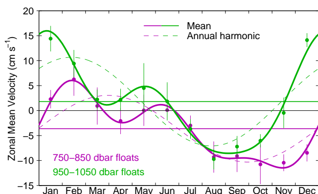
Figure 5 Harmonic analysis of the monthly zonal mean currents within one degree of equator. Dots and vertical bars indicate monthly mean values and their errors. Thick curves give the synthesis using the mean, annual, semi-annual and fourthmonthly harmonics.
