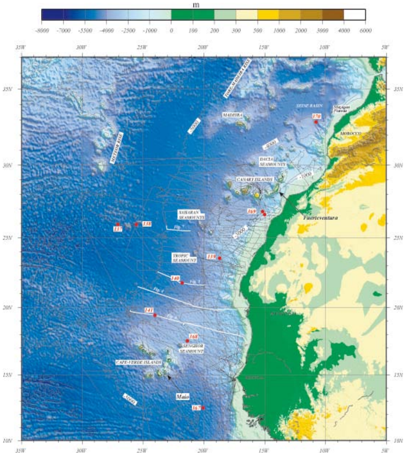
1) General bathymetric and situation map (from Gibraltar to the Sierra Leone) showing the reflection seismic data and the DSDP holes used in this study.
