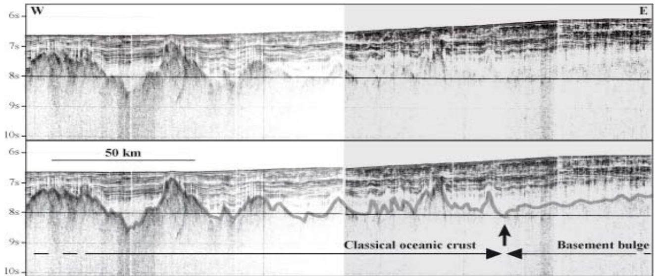
8) Detail of a seismic reflection profile and its interpretation (localisation see figure 1 or 3). The basement reflector is typically oceanic (very rough) at the left hand side. It is smoother at the right hand side, though still slightly chaotic, typical of the basement bulge area.
