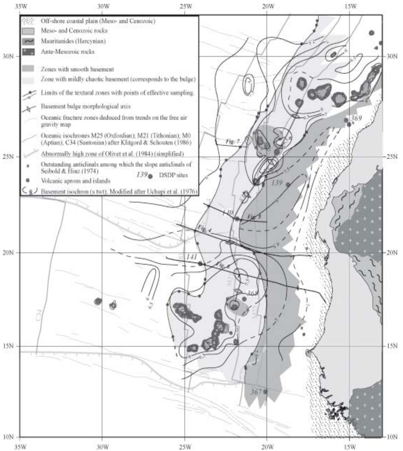
3) Structural map and localisation of the basement bulge based on seismic-reflection.
