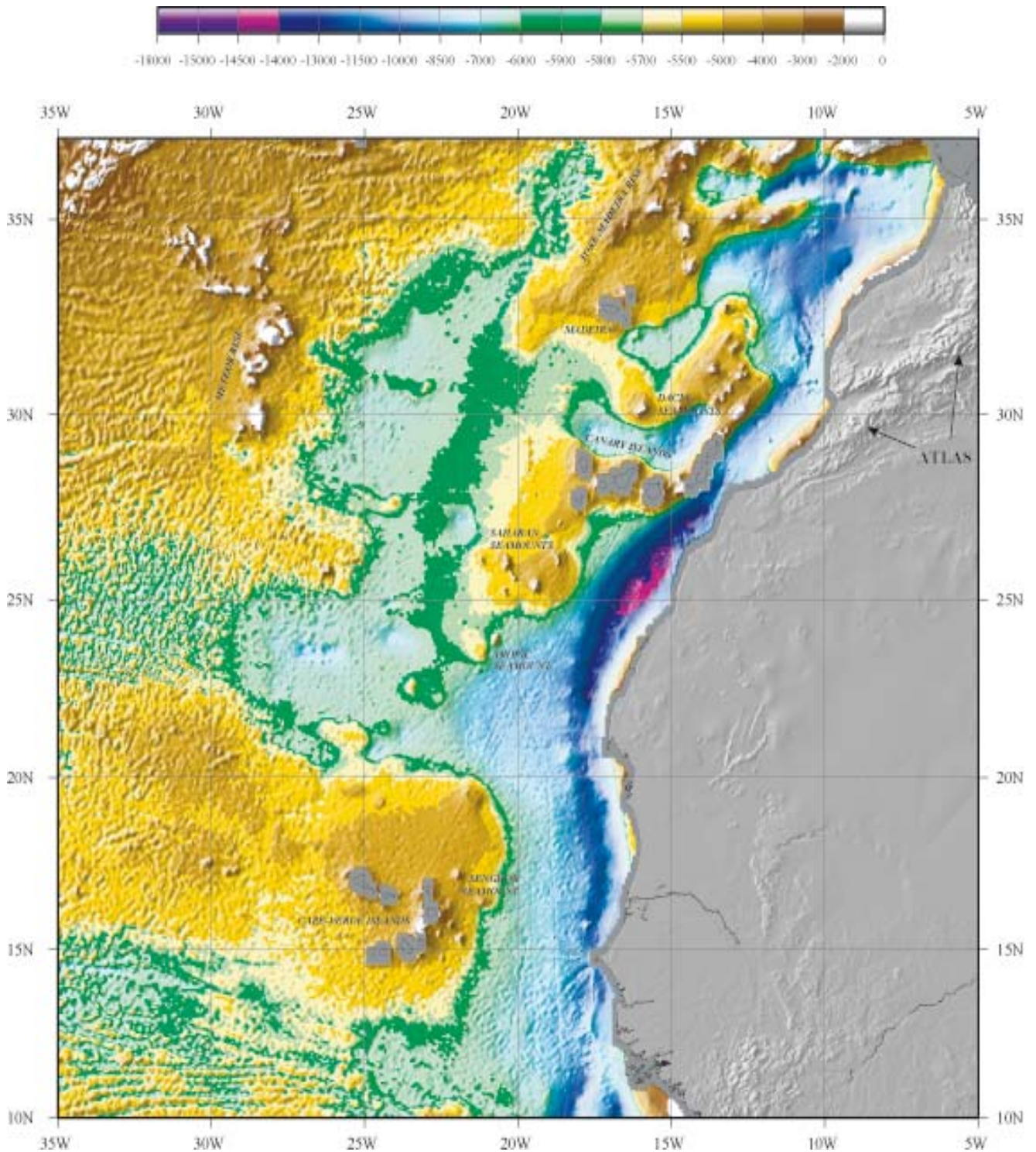
4) Map of the basement calculated by subtracting the thickness of sediments, coming from the digital database of the NGDC "total sediment thickness database for the world's oceans and marginal seas", from the bathymetry.
