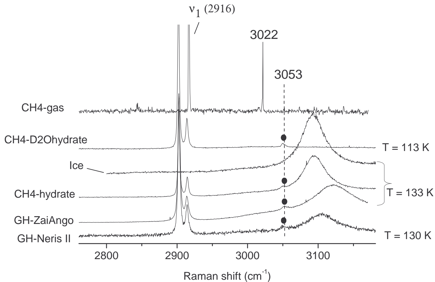
FIGURE 3: Comparative spectra of the O-H spectral region of water at \sim 3100 \text{ cm}^{-1} . The weak additional component at \sim 3053 \text{ cm}^{-1} characterizes the presence of hydrates. It is assigned to an overtone of methane (see text). Its presence is confirmed on the spectra of the \text{CH}_4 -deuterohydrate where the contribution of water molecules (O-D stretching) are absent from the spectral region. Variations in the O-H band position is due to differences in temperature and/or reflect the structural differences between ice and hydrate which are both present in variable amounts under the laser spot. The spectra of methane in the free gas phase is shown for comparison (see discussion).
