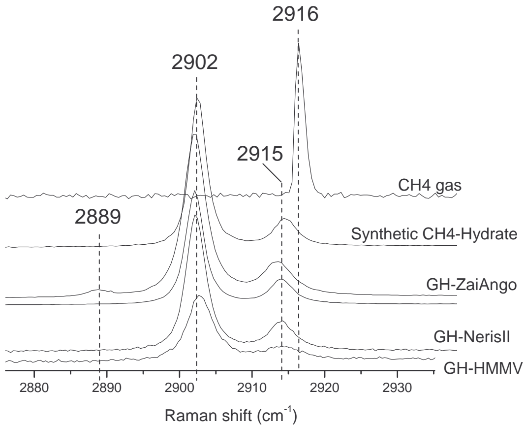
FIGURE 2: Comparison between Raman spectra of natural hydrates collected at different sites and synthetic CH 4 -hydrate. The spectral region corresponds to the C-H stretching of methane. The characteristic twin bands at ~ 2902 and ~ 2915 cm -1 are attributed to CH 4 trapped in the large and small cage of the type I structure. C-H stretching of methane gas (atmospheric pressure) with a unique band at ~ 2916 cm -1 is plotted for comparison. Note the occurrence of a component at ~ 2889 cm -1 attributed to C-H stretching of CH, CH 2 , CH 3 group of aliphatic groups.
