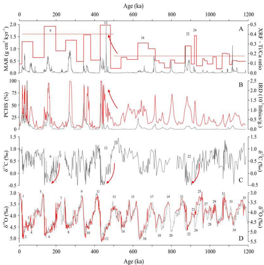
Figure 2 Summary of the data obtained from site MD01-2448. A. Terrigenous Mass Accumulation Rates (MAR, continuous red line; glacial average MAR for MIS 34-14 and MIS 12-2 intervals, dashed red line) and X-ray fluorescence (XRF) Ti/Ca ratio (continuous grey line); B. Abundance of the polar planktic foraminifera Neogloboquadrina pachyderma senestral (PCHS, continuous red line) and ice-rafted detritus (IRD) content (continuous grey line); C. Benthic \delta^{13}\text{C} ; d. Benthic \delta^{18}\text{O} for core MD01-2448 (continuous red line) synchronized onto the LR04 benthic oxygen isotope stack 30 (dashed black line) using the marine isotope stage (MIS) boundaries proposed in ref. 30 as tie-points. Stable isotope
