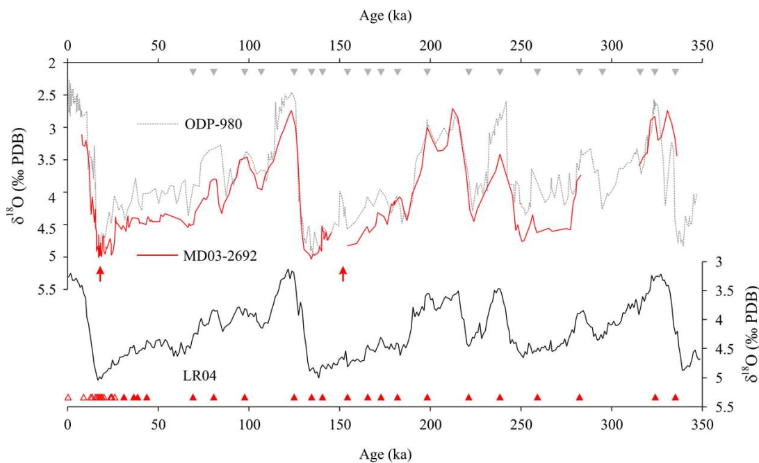
Figure 4. Basis of the age models for cores MD03-2692 and ODP-980. Age control were established by alignment of the benthic foraminifera oxygen isotope records ( \delta^{18}\text{O} (‰), continuous red line: MD03-2692 and dotted grey line: ODP-980 (McManus et al., 1999)) with the LR04 benthic oxygen isotope stack of Lisiecki and Raymo (2005). Age model for core ODP-980 is similar to those published by McManus et al. (1999) between 60 and 0 ka. Filled red and grey triangles indicate positions of the tie points for cores MD03-2692 and ODP-980, respectively. Open red triangles indicate the position of the AMS ^{14}\text{C} datings for core MD03-2692. Red arrows indicate the position of the laminated facies in core MD03-2692.
