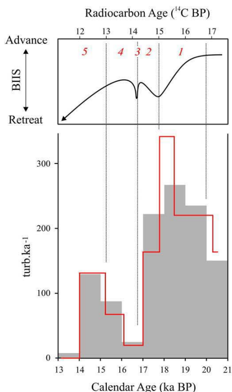
Fig. 11. Comparison between turbidite deposit frequency in the Celtic turbidite system (core MD04-2836) (this study) and the BIIS oscillations in the Irish Sea Basin (McCabe et al., 2007b). Continuous red line show the frequency of turbidite deposits ( \text{turb ka}^{-1} ) between two consecutive control points of the age model of core MD04-2836 while the histogram show the turbidite deposit frequency using a time slicing of 1 ka. 1: 'Cooley Point Interstadial' (from \geq 16.7 to \leq 15 ^{14}\text{C} ka BP); 2: 'Clogher Head Stadial' (from \geq 15 to \leq 14.2 ^{14}\text{C} ka BP); 3: 'Llins Interstadial' ( \sim 14.2 ^{14}\text{C} ka BP); 4: 'Killard Point Stadial' (from \geq 14.2 to \sim 13.0 ^{14}\text{C} ka BP); 5: 'Rough Island Interstadial' (after \sim 13.0 ^{14}\text{C} ka BP) (McCabe et al., 2007b). Note the close relationship between the main retreat periods of the BIIS and enhanced turbiditic activity in the Whittard channel. (For interpretation of the references to colour in this figure legend, the reader is referred to the web version of this article.)
