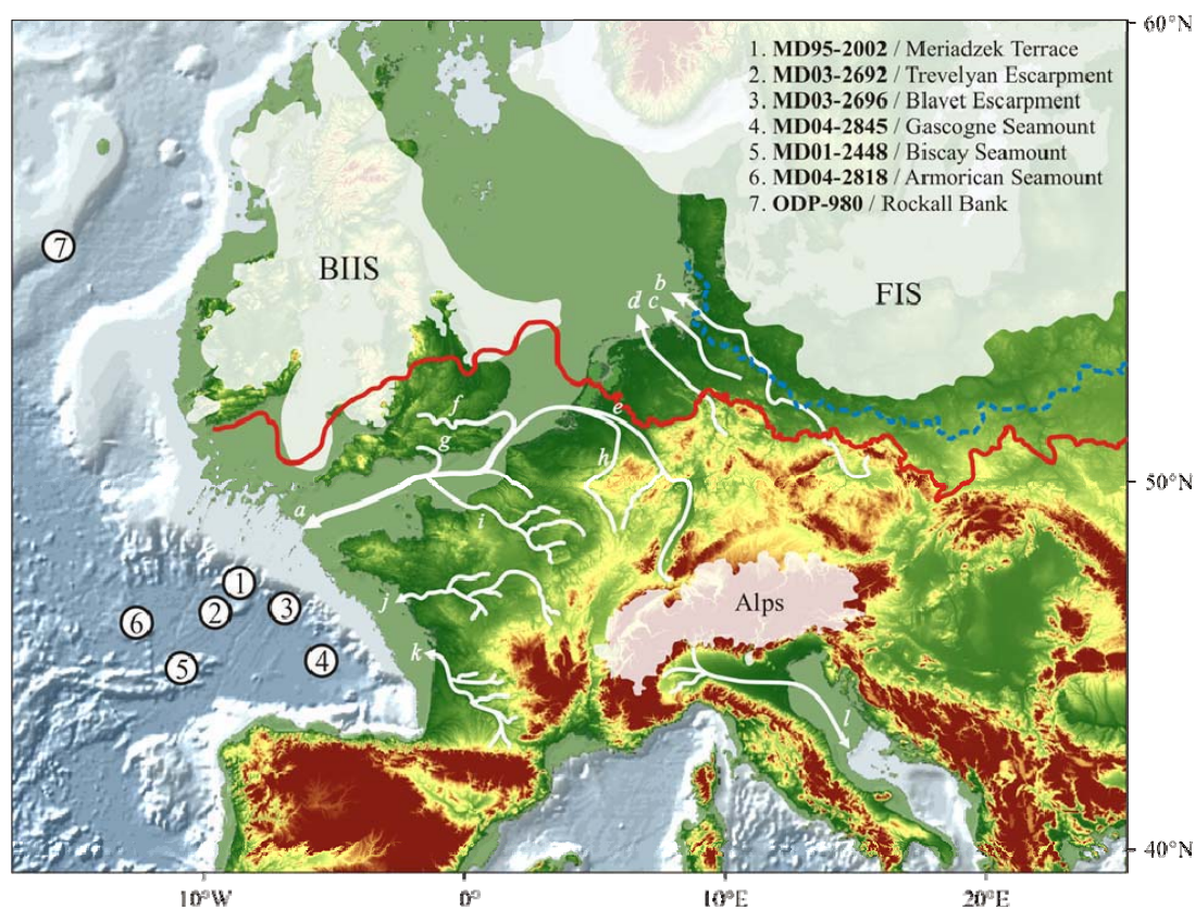
Figure 1. Map of NW Europe showing the glacial limits of the British-Irish Ice Sheet (BIIS), Fennoscandian Ice Sheet (FIS) and the Alps Glaciers for the Late Weichselian (MIS 2 - white shaded area) and Saalian glaciations (Drenthe advance = continuous red line; Warthe advance = dotted blue line) (Ehlers and Gibbard, 2004). The white arrows and the associated lowercase letters identify the main European rivers: a: ‘Fleuve Manche’, b: Elbe, c: Weser, d: Ems, e: Rhine, f: Thames, g: Solent, h: Meuse, i: Seine, j: Loire, k: Gironde, l: Pô. The numbers indicate the core locations. Bathymetry and altimetry correspond to the ETOPO2 ( http://www.ngdc.noaa.gov/mgg/fliers/01magg04.html ) and SRTM (Global Land Cover Facility, http://www.landcover.org ) data, respectively.
