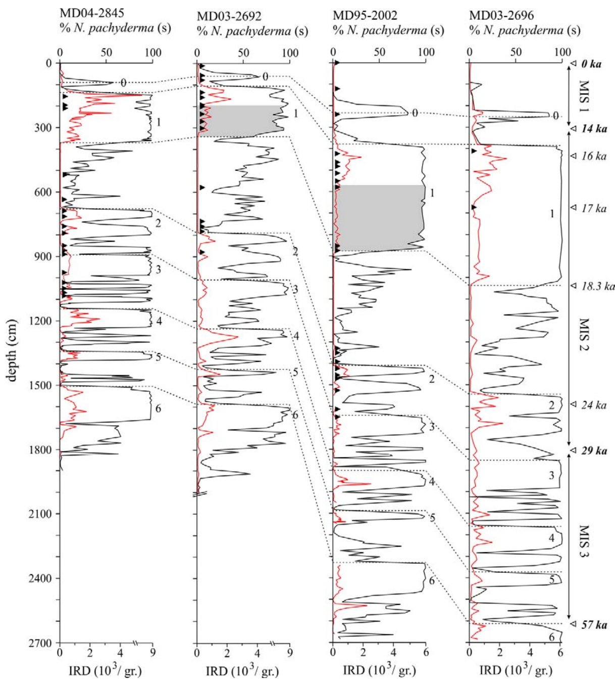
Figure 2. Abundance of planktic foraminifera N. pachyderma (s) (continuous black line - %) and of IRD (red line - 10^3/\text{gr.} ) from sediment cores MD04-2845, MD03-2692, MD95-2002 and MD03-2696. Dashed black lines and associated numbers represent core-to-core correlations using the upper limit of the Heinrich events (HE) 0 (i.e. Younger Dryas), HE 2, HE 3, HE 4, HE 5 and HE 6 and the lower and upper limits of the HE 1. AMS 14C dated samples are marked by black triangles on the depth scale. Bold ages and associated open triangles delimit the Marine Isotope Stages (MIS) boundaries according to the chronology of Lisiecki and Raymo (2005). Intermediate ages and associated open triangles within the MIS 2 make reference to the ages used in the Figure 6. Grey shading corresponds to the laminated facies deposited between ca. 18.3 and ca. 17 ka at site MD03-2692 and MD95-2002.
