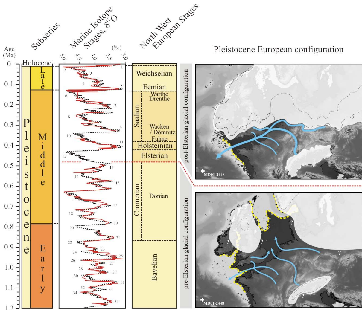
Figure 3 Correlation between the European continental glaciation-derived chronology (North West European Stages 3 ) and the marine isotope stratigraphy (dotted black line: LR-04 stack 30 ; continuous red line: benthic \delta^{18}O for core MD01-2448; MIS are labelled) based on sedimentary evidence from core MD01-2448 (for details see text). In the later Middle Pleistocene pre-Elsterian period (lower panel), the British and Fennoscandian ice-sheets remained isolated during glacial intervals, and usually restricted to mountainous areas (dashed black line). The exception was the Donian glaciation (MIS 16) during which the ice sheets (white-shaded areas), although more extensive, remained separated. The British and Fennoscandian ice-sheets were confluent for the first time, in the North Sea basin during the Elsterian glaciation, MIS 12 (upper panel). This caused a massive proglacial lake to form in the basin, the catastrophic drainage of which caused initial breaching of the Weald-Artois structural barrier ca. 455 ky ago. Subsequently, whenever the European ice-sheets advanced during later glaciations, the North Sea fluvial system could be directed southwards during lowstand conditions. Such a condition certainly occurred during the Saalian (MIS 6, continuous black line) and Weichselian (MIS 2, dashed black line) maximum ice-advances. The glacial shoreline is represented by the discontinuous yellow lines.
